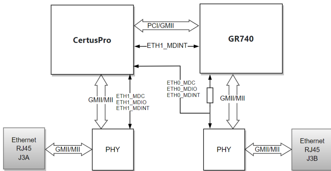
Figure 4-26 GMII/MII Intercommunication
