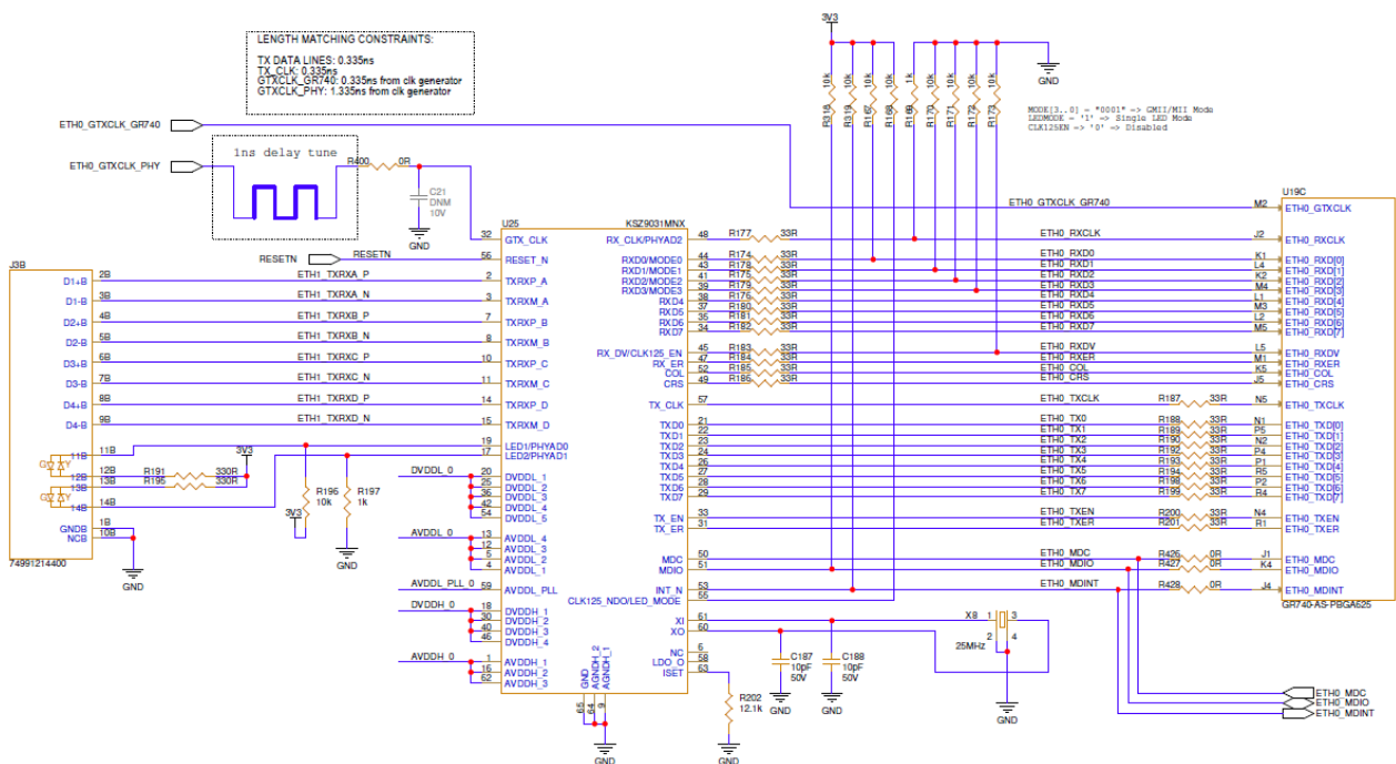
Figure 4-15 ETH0 implementation
