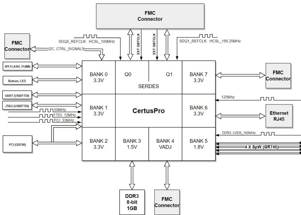
Figure 4-17 CertusPro-NX implementation
