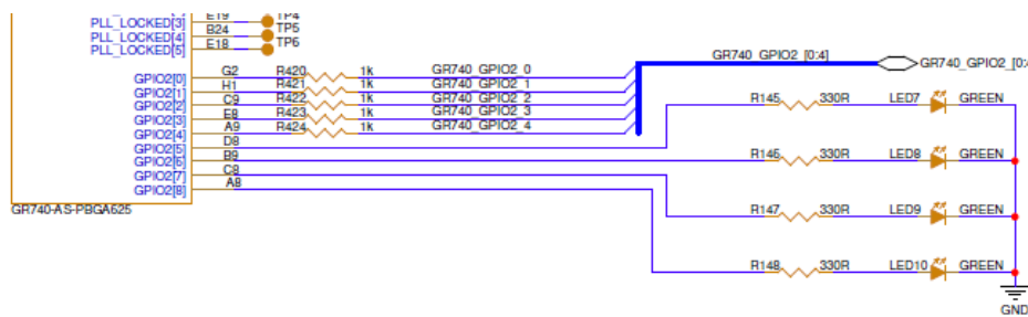
Figure 4-16 GPIO for GR740
