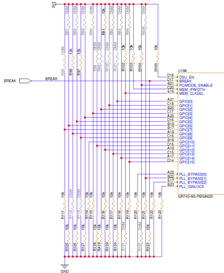
Figure 4-10 Bootstrap signals
