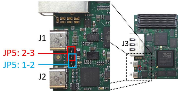
Figure 4-4 Jumper Configuration
