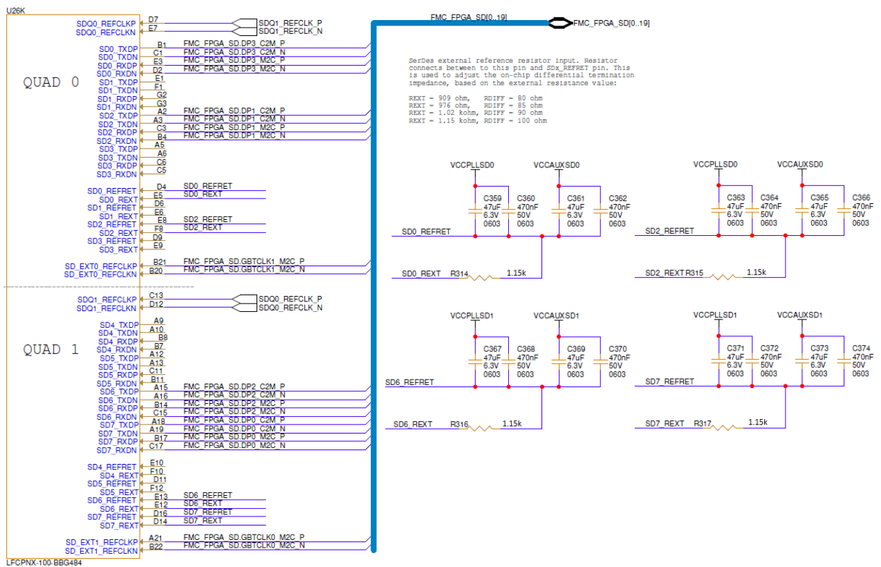
Figure 4-24 SerDes implementation
