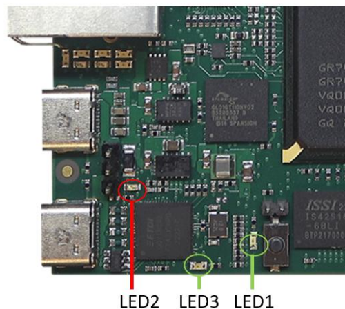
Figure 4-5 LED(1-3) board placement
