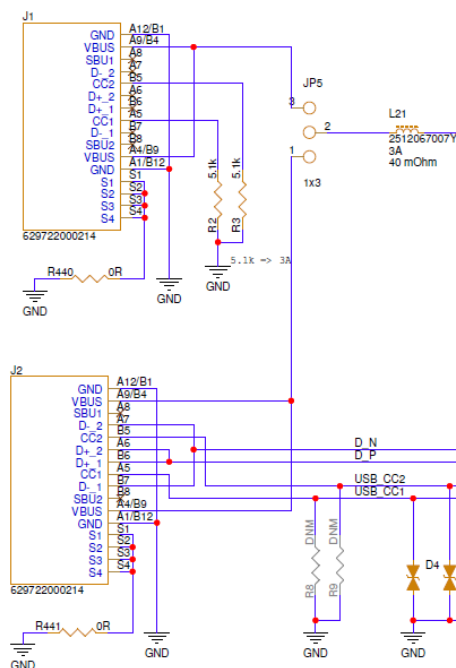
Figure 4-3 USB-C connector for power supply solution
