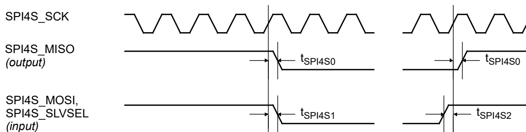
Figure 13. SPI interface timing waveforms
