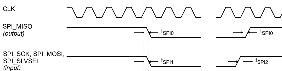
Figure 12. SPI interface timing waveforms
