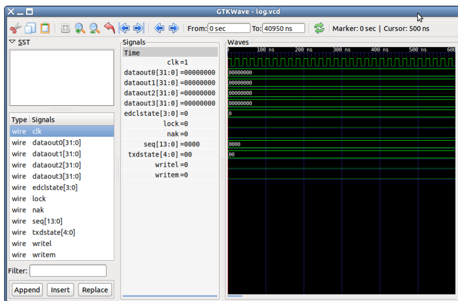
Figure 6.1. GTKWave
