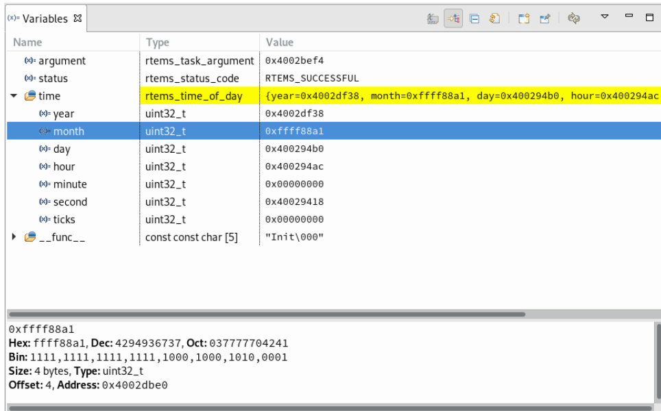
Figure 4.32. The Variables view showing the symbols of the currently active stack frame. Here, month, an uint32_t is selected, which belongs to the time variable, which is of rtems_time_of_day type. We see that month has value 0xffff88a1, is 4 bytes, has an offset of 4 from the parent type and resides at address 0x4002dbe0.
