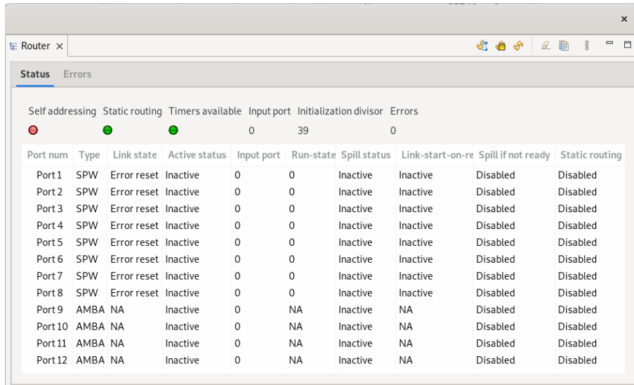
Figure 4.13. Router view
