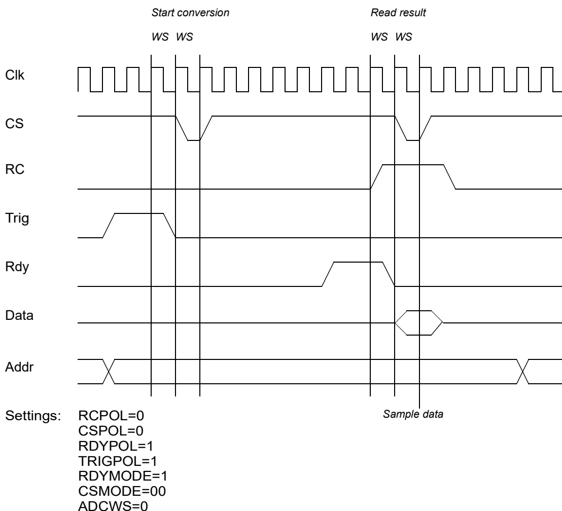
Figure 129. Analogue to digital conversion waveform, 0 wait states (WS)
