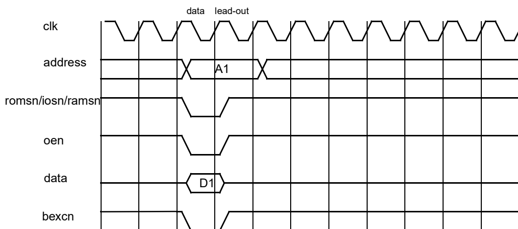
Figure 98. Read cycle with BEXCN.
