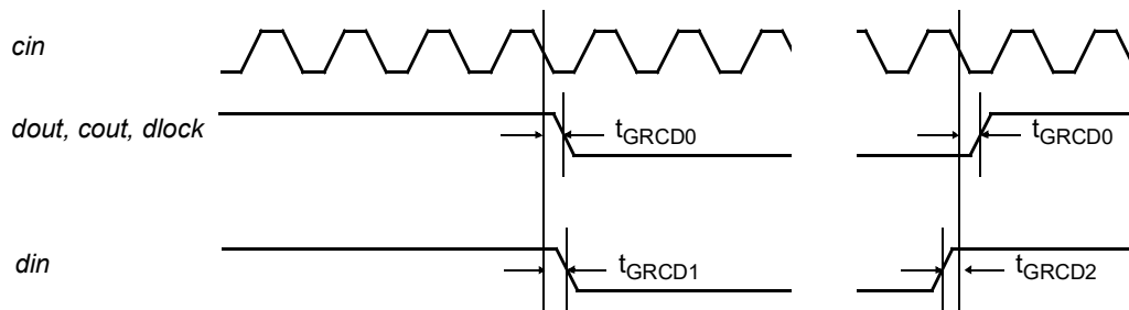
Figure 361. Timing waveforms - GRCD
