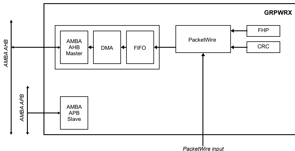
Figure 385. Block diagram
