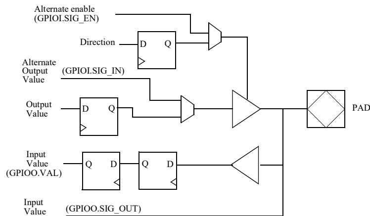
Figure 149. General Purpose I/O Port diagram
