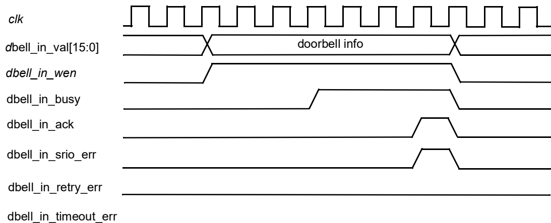
Figure 230. Skew and jitter timing waveforms
