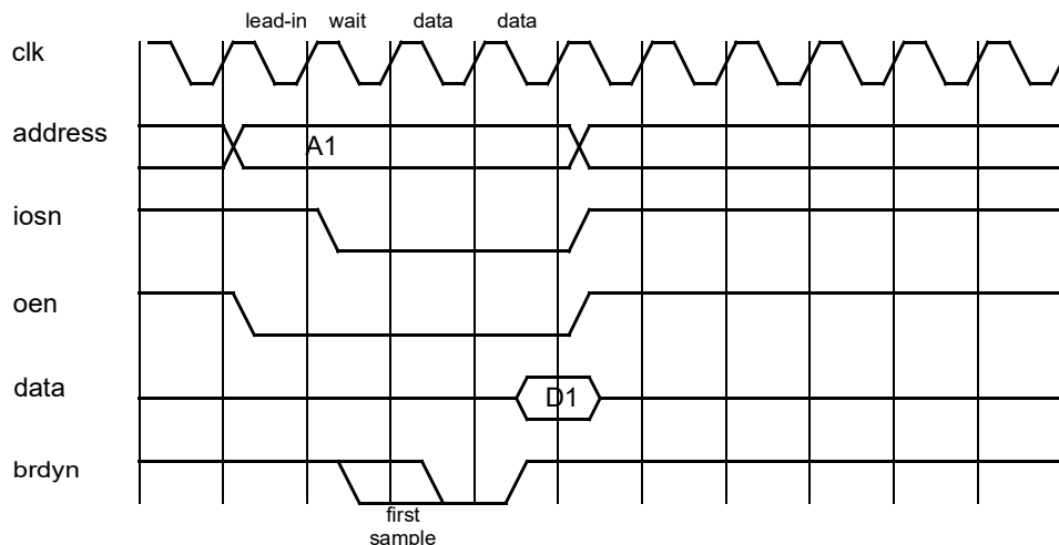
Figure 100. I/O READ cycle, programmed with 1 wait state, and with an extra data cycle added with BRDYN.
