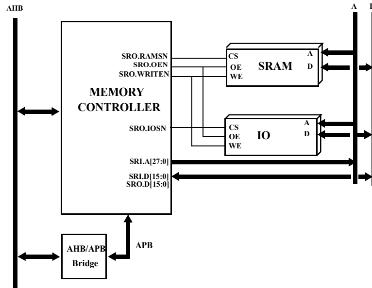
Figure 111. Block diagram
