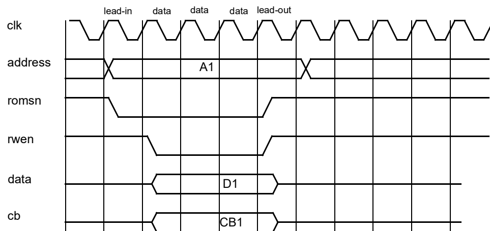
Figure 285. Prom write cycle (2-waitstates)
