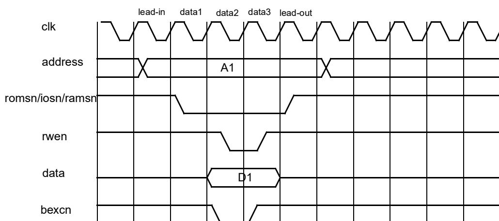
Figure 99. Write cycle with BEXCN.
