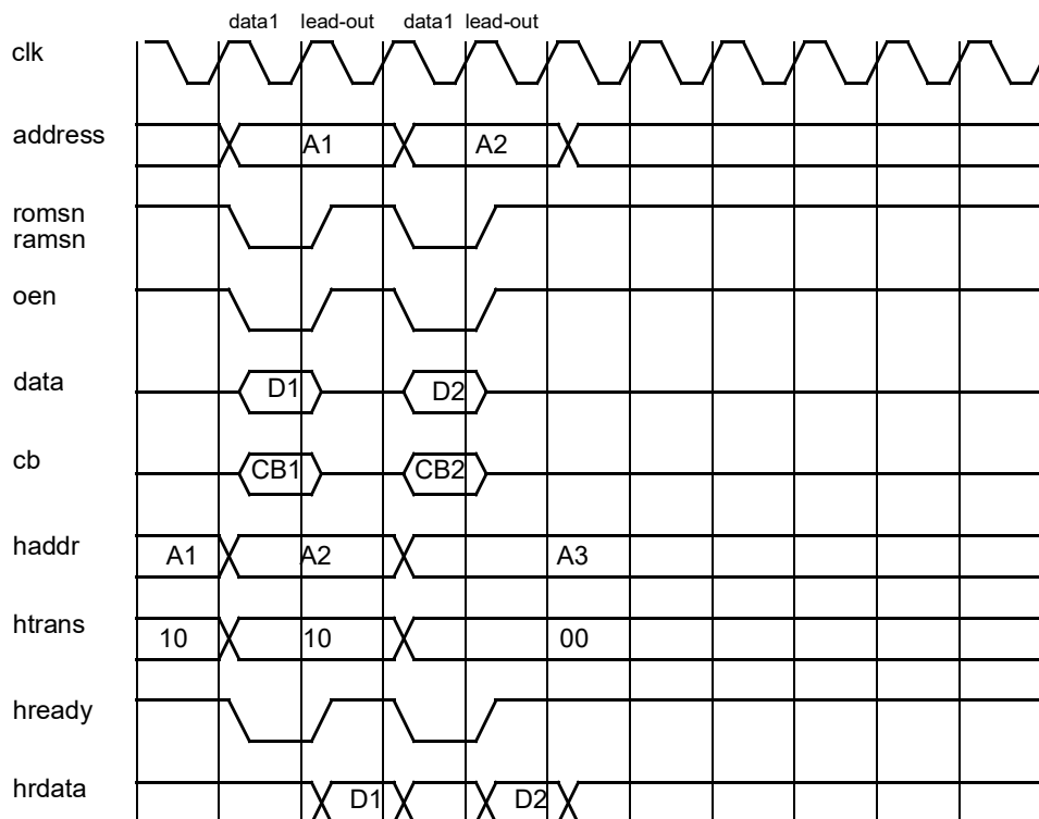
Figure 101. PROM/SRAM non-consecutive read cycles.
