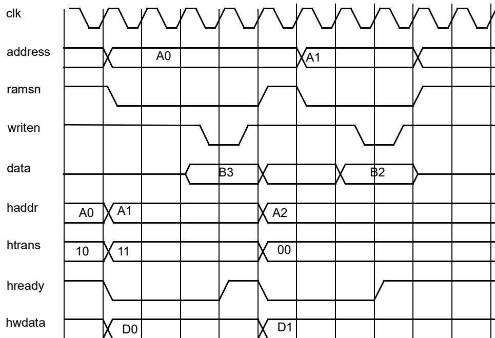
Figure 115. 8-bit SRAM non-sequential write access with 0 wait-states and EDAC enabled.
