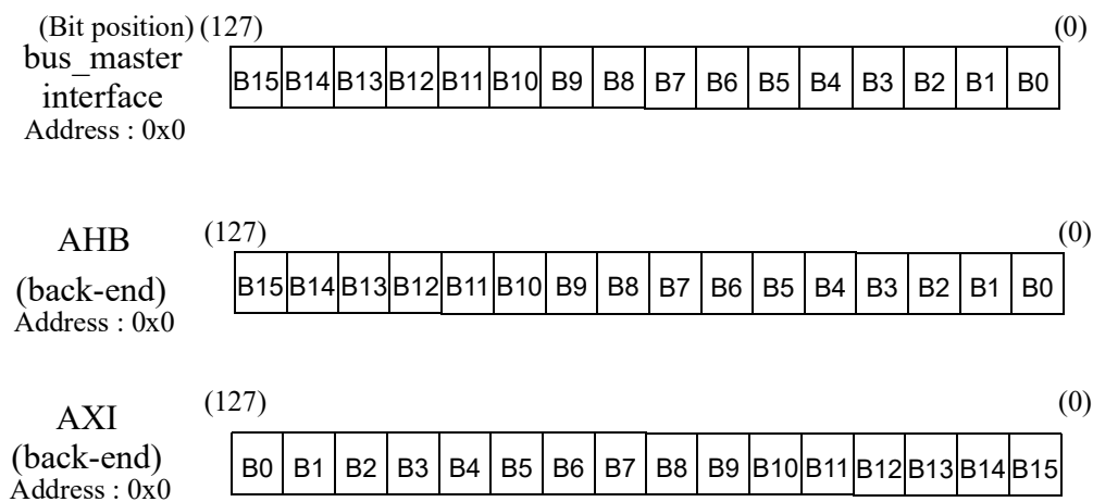
Figure 227. 16 Byte Access on AHB and AXI back-ends (BM_DW=128-bit, BE_DW=128-bit)
