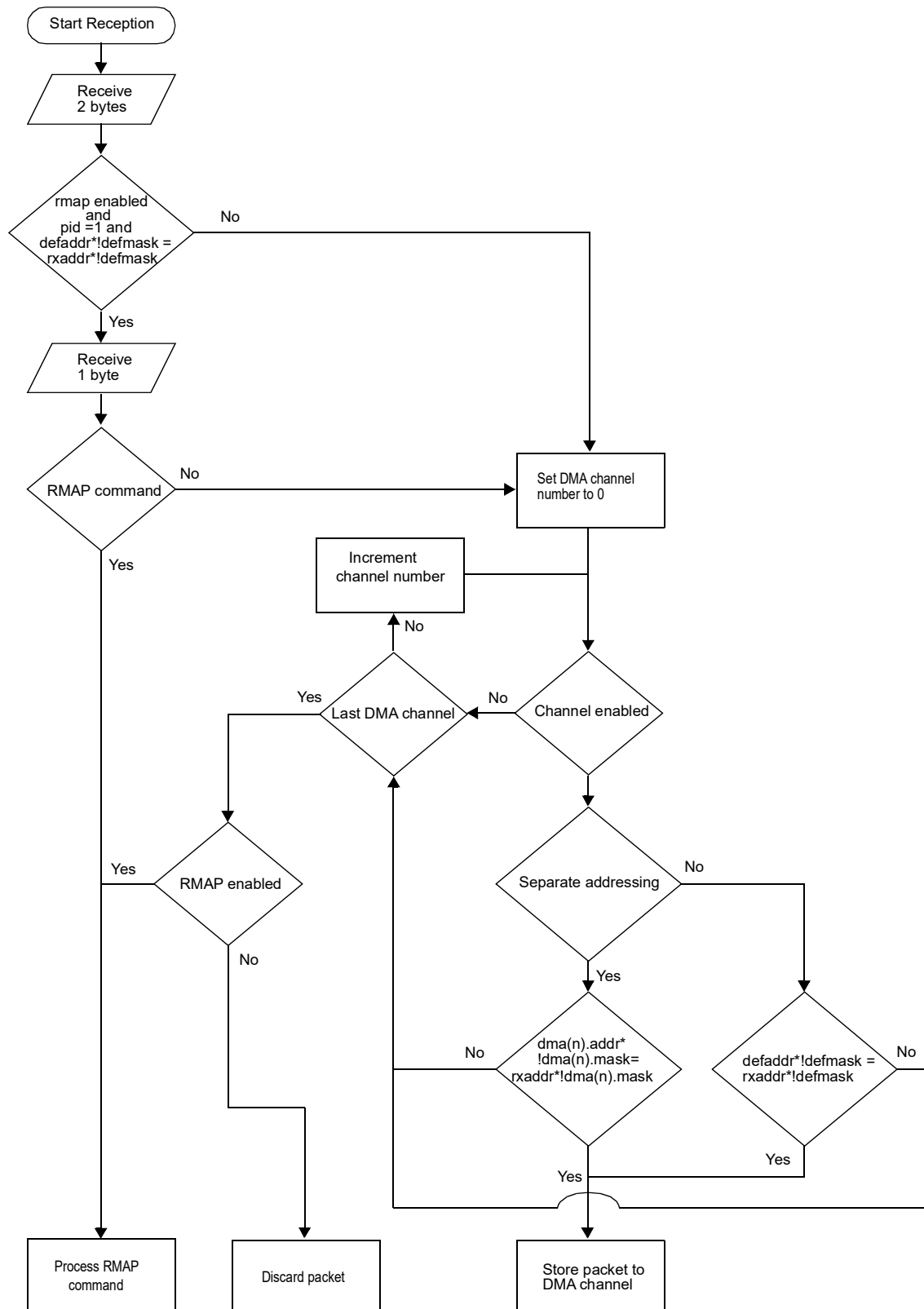
Figure 222. Flow chart of packet reception (promiscuous mode disabled).
