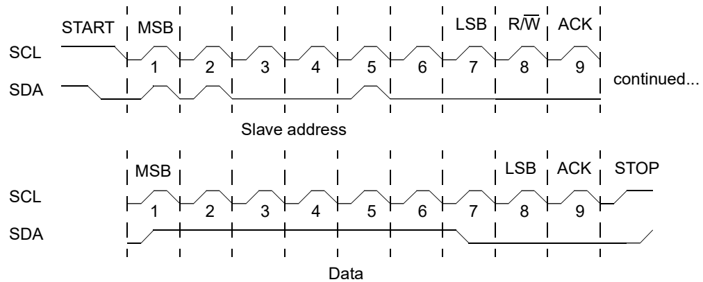
Figure 248. Complete I 2 C data transfer
