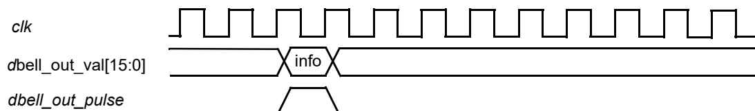
Figure 231. Skew and jitter timing waveforms
