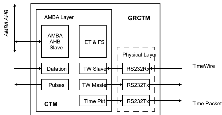
Figure 378. Block diagram
