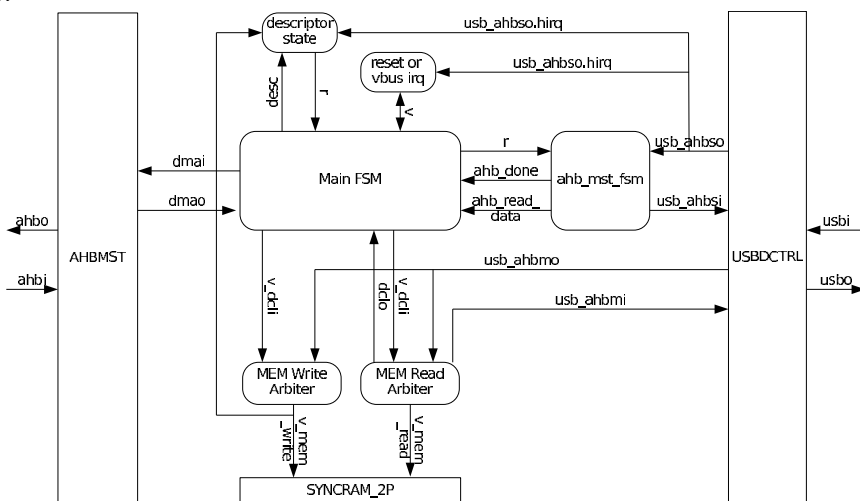
Figure 237. Block diagram of the internal structure of the GRUSBDC. Blocks with rounded corners are implemented as VHDL procedures while squares represent VHDL entities.
