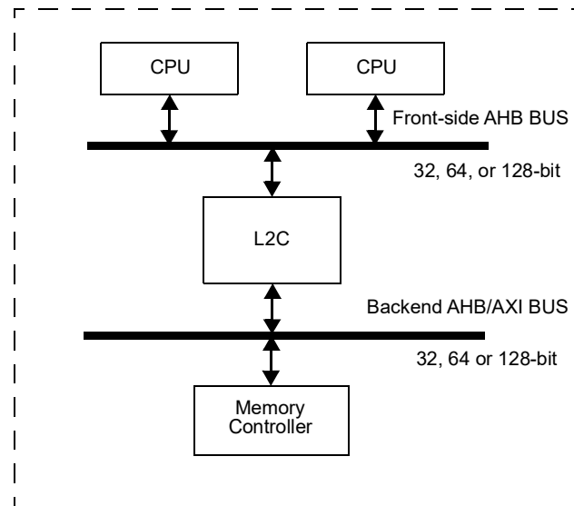
Figure 257. Block diagram
