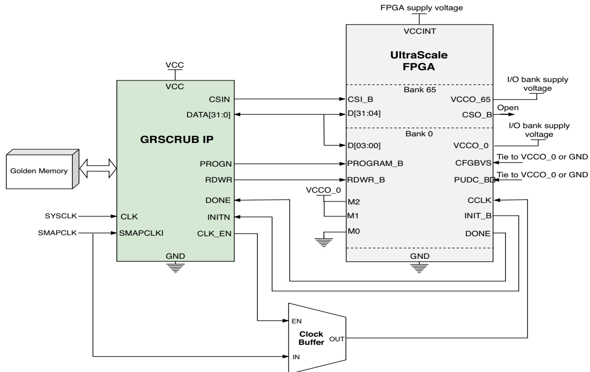
Figure 172. Example of GRSCRUB and slave SelectMap interface connection for Xilinx UltraScale FPGA
