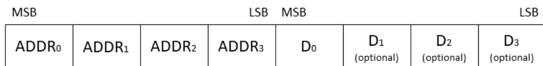
Figure 136. Use of data bytes in write commands (RPDO1 and RPDO3)
