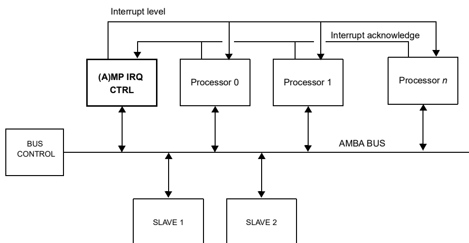
Figure 254. LEON multiprocessor system with Multiprocessor Interrupt controller
