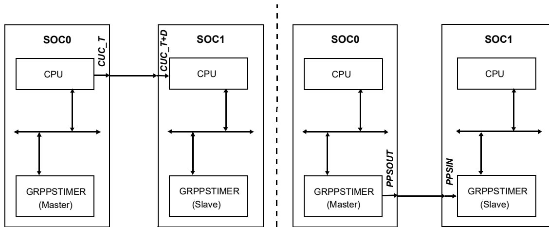
Figure 165. Two strategies to synchronise two GRPPSTIMERS
