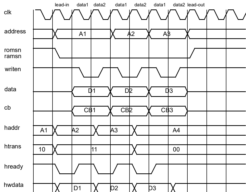
Figure 106. 32-bit PROM/SRAM sequential write access with 0 wait-states and EDAC disabled.
