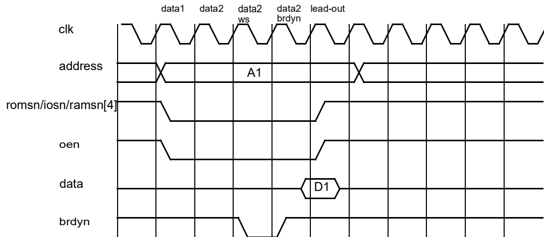
Figure 293. Read cycle with one waitstate (configured) and one BRDYN generated waitstate (synchronous sampling).
