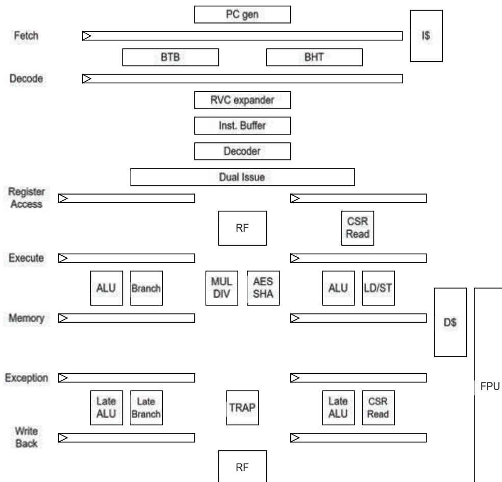
Figure 305. NOEL-V integer unit datapath diagram
