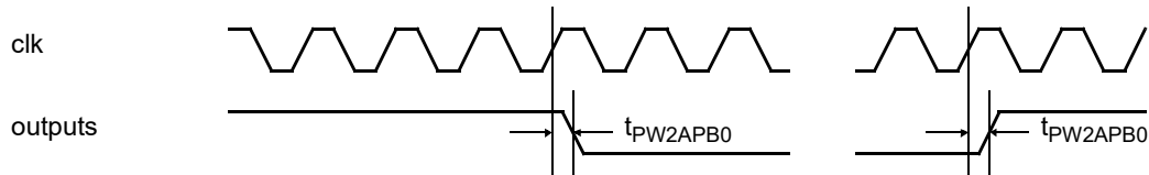
Figure 393. Timing waveforms
