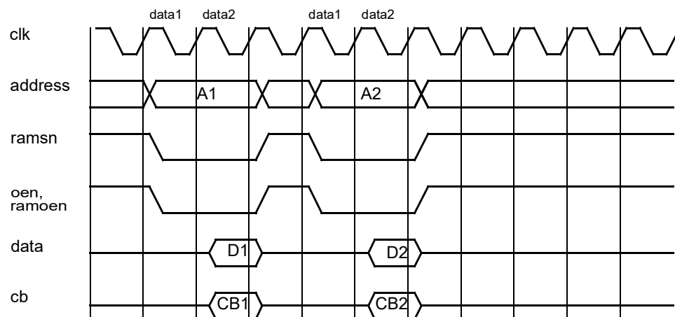
Figure 82. Sram non-consecutive read cycles.
