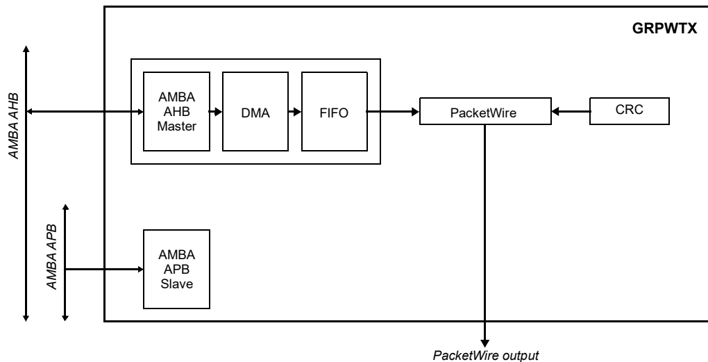
Figure 388. Block diagram
