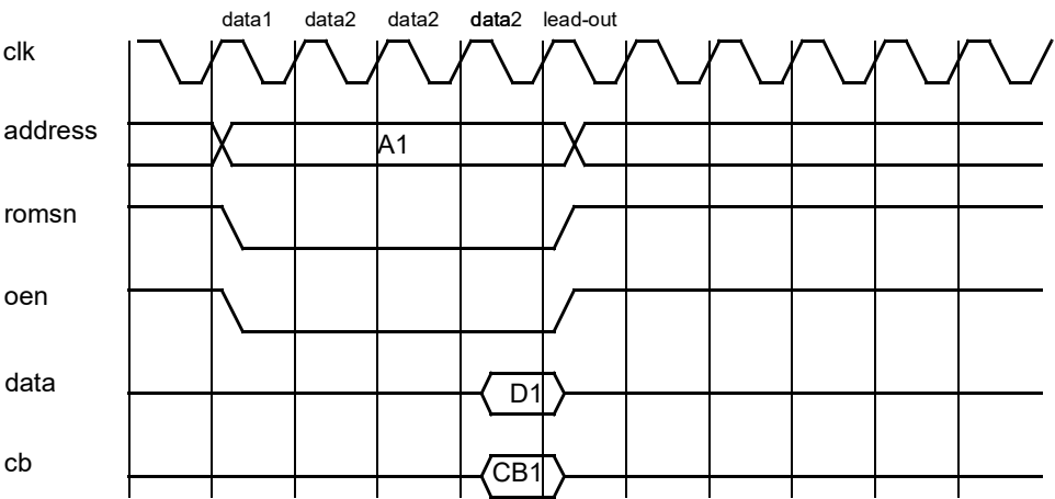
Figure 283. Prom read access with two waitstates.
