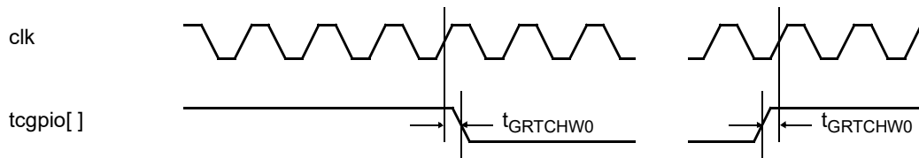
Figure 373. Timing waveforms
