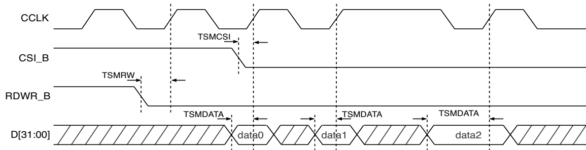
Figure 176. SelectMap timing characteristics for data loading to FPGA
