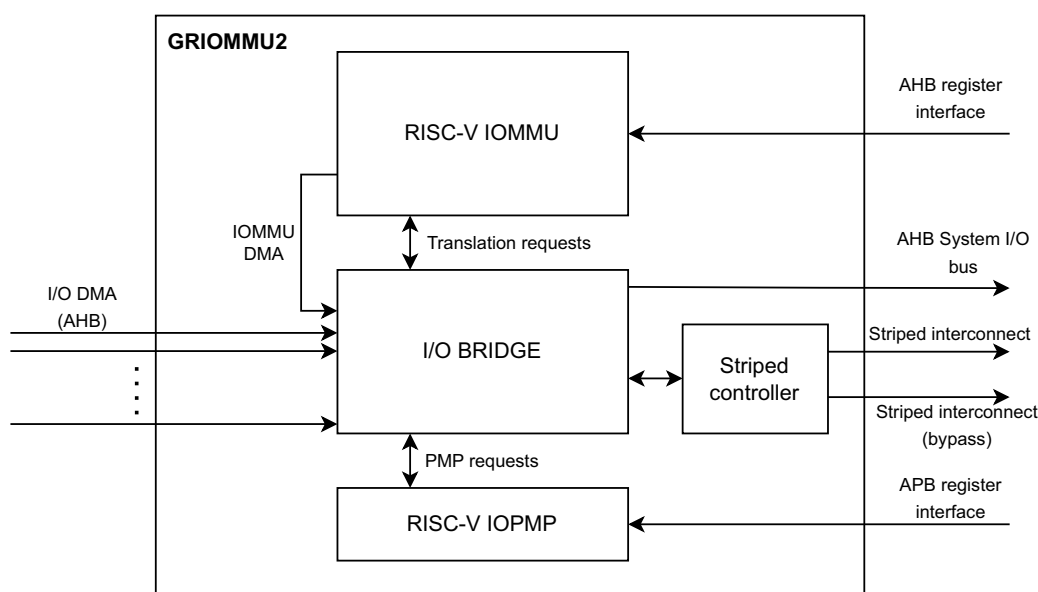
Figure 153. Block diagram of GRIOMMU2 using the higher throughput striped AHB interconnect bridge.
