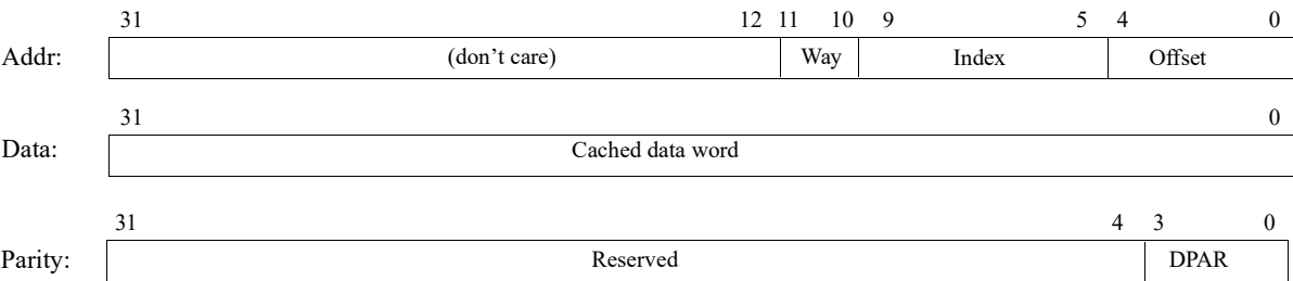
Figure 261. ASI 0xC-0xF address mapping and data layout
