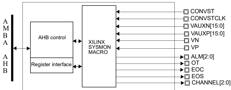
Figure 232. Block diagram
