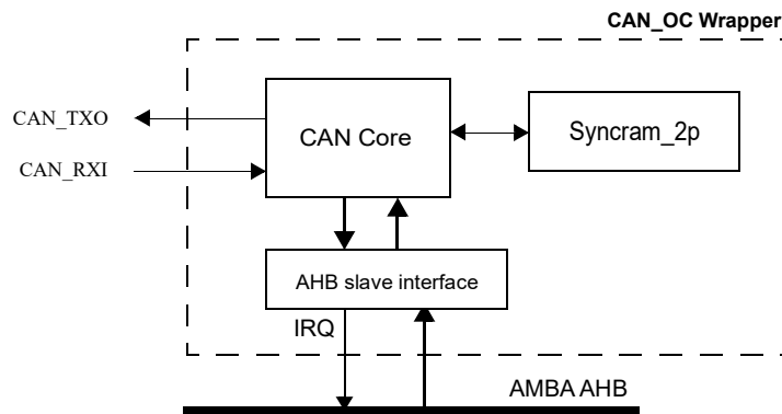
Figure 37. Block diagram
