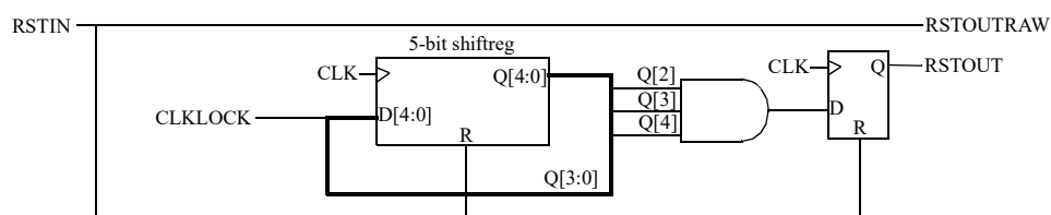
Figure 314. Reset generator with VHDL generic syncrst set to 0 and scan test disabled
