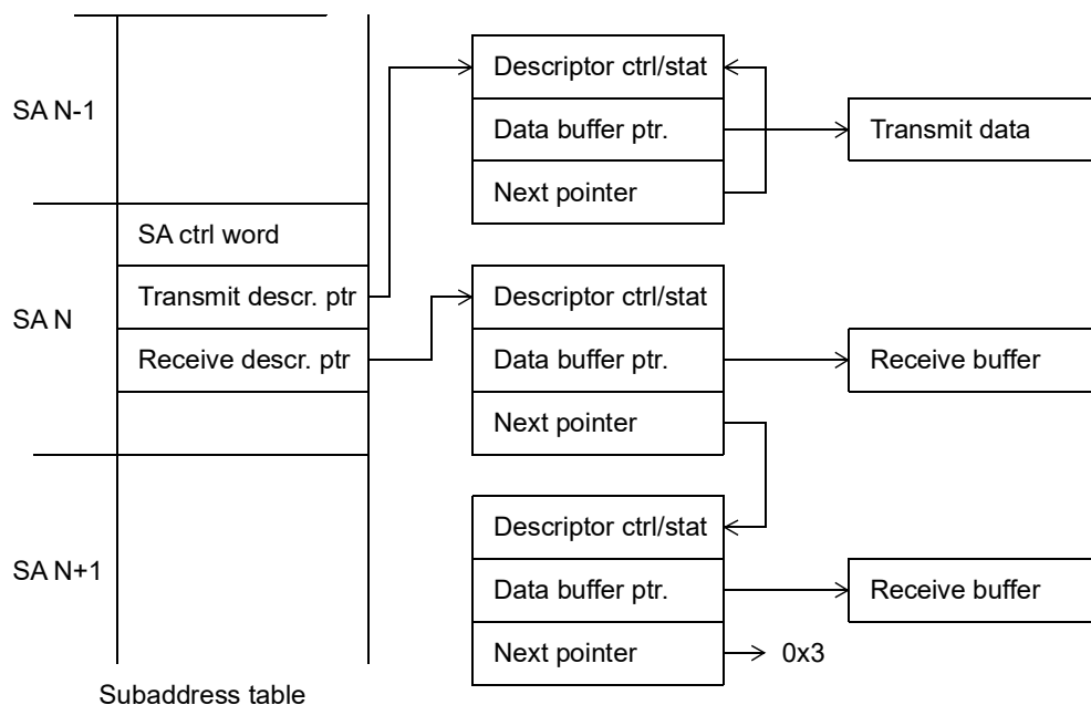
Figure 123. RT subaddress data structure example diagram
