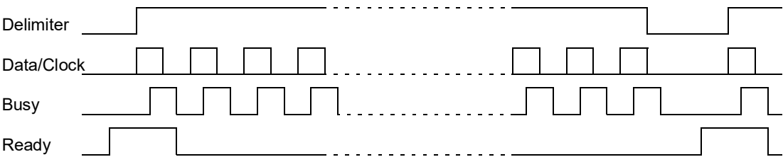
Figure 392. Handshake with ready signalling
