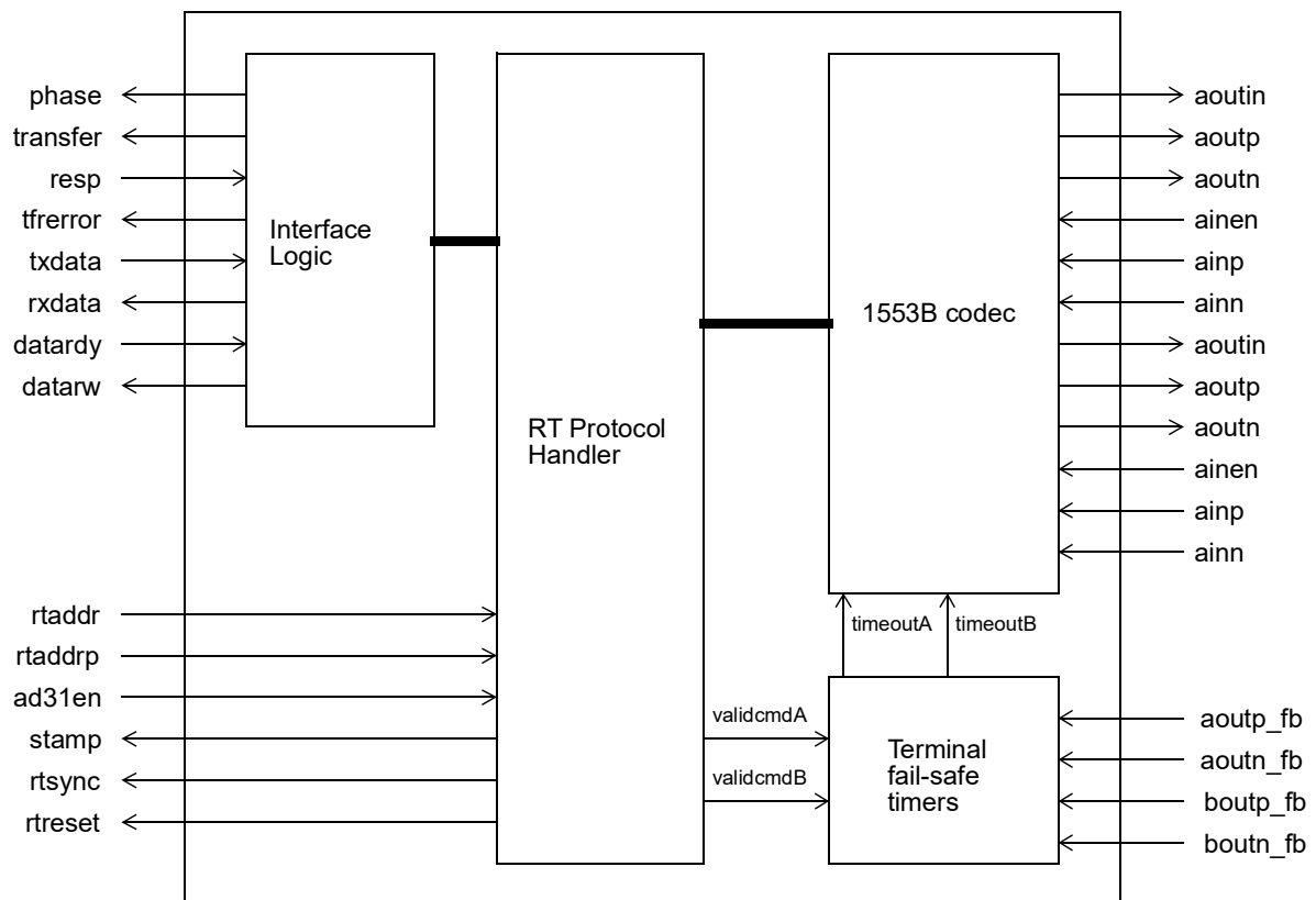
Figure 169. GRRT block diagram showing interfacing signals
