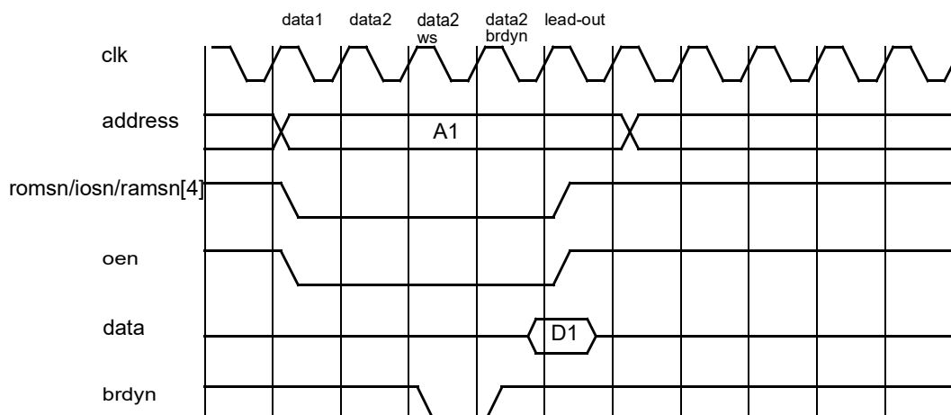
Figure 89. Read cycle with one waitstate (configured) and one BRDYN generated waitstate (synchronous sampling).
