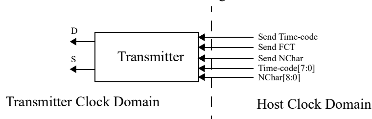
Figure 190. Schematic of the link interface transmitter.
