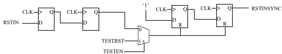
Figure 316. Extra Reset generator logic with VHDL generic syncin set to 1 to synchronize input reset and scan test enabled
