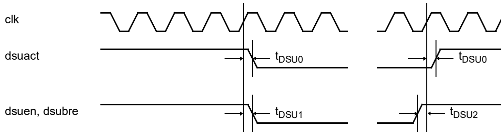
Figure 68. Timing waveforms
