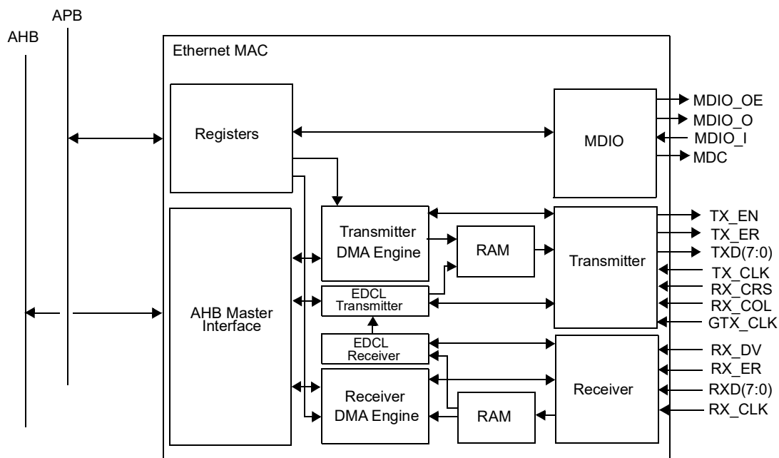
Figure 141. Block diagram of the internal structure of the GRETH_GBIT.
