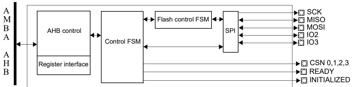
Figure 326. Block diagram
