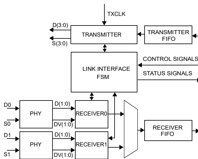
Figure 204. Block diagram
