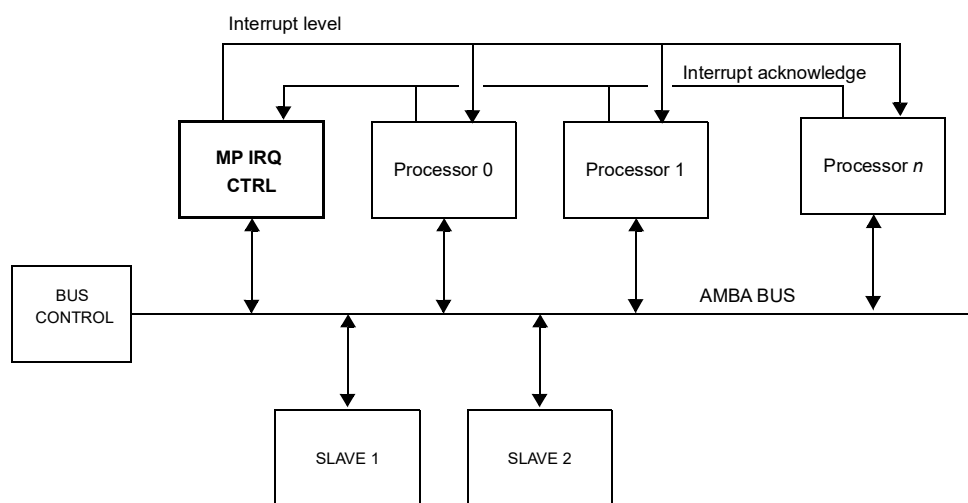
Figure 252. LEON multiprocessor system with Multiprocessor Interrupt controller
