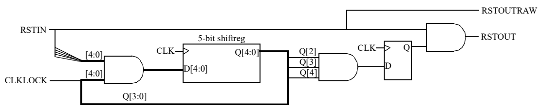
Figure 313. Reset generator with VHDL generic syncrst set to 1
