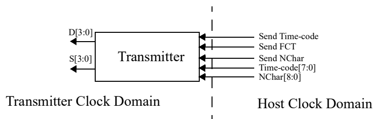
Figure 205. Schematic of the link interface transmitter. Some bits in D[3:0] and S[3:0] may be unused, depending on the values of the output_type , and ports VHDL generics (see section 80.8).
