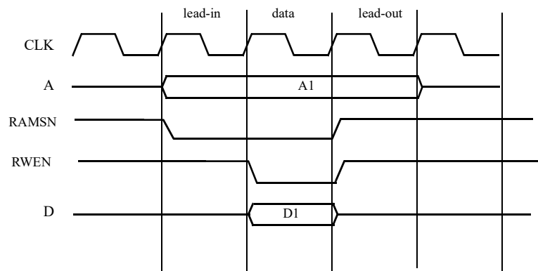
Figure 334. 32-bit PROM/SRAM/IO write cycle
