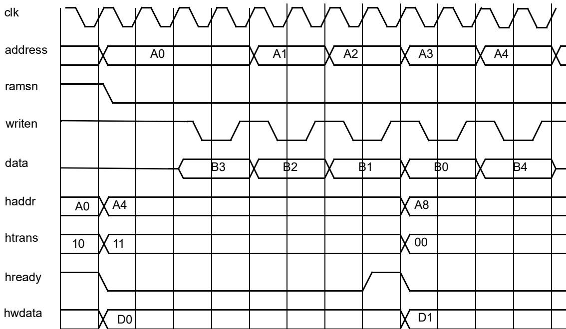
Figure 114. 32-bit SRAM sequential writeaccess with 0 wait-states and EDAC enabled.
