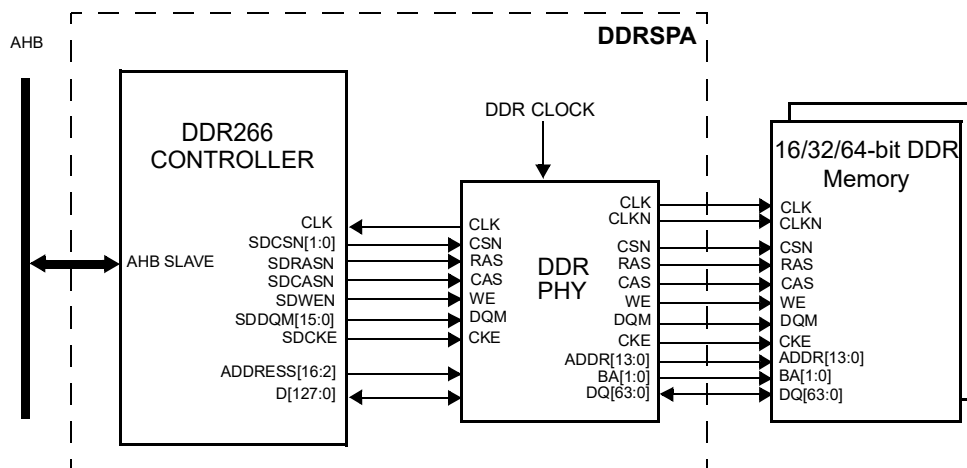
Figure 65. DDRSPA Memory controller connected to AMBA bus and DDR SDRAM
