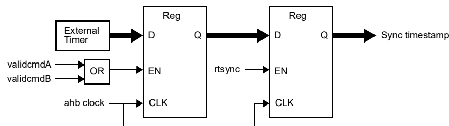
Figure 126. Obtaining an RT sync timestamp in hardware with an external time base
