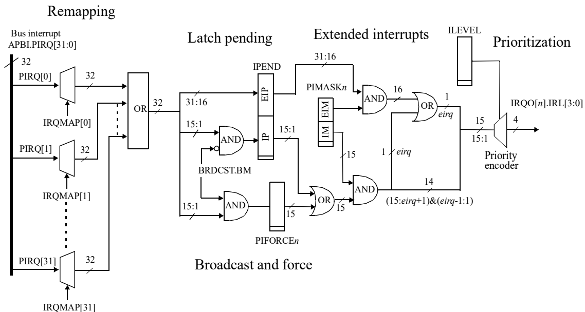
Figure 253. Interrupt controller block diagram. Interrupt acknowledgement is not shown. Logic is only shown for one processor. When multiple processors are implemented ( ncpu > 1 ), the interrupt forcing, masking, and priority encoding is performed separately for each processor. Each processor has its own PIFORCE_n and PIMASK_n register. The registers IRQMAP , IPEND , BRDCST , and ILEVEL are common to all processors. Interrupt remapping and extended interrupts are optional features that can be disabled at implementation time to reduce complexity.
