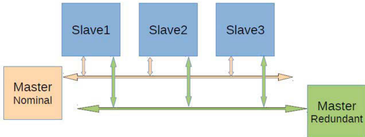
Figure 331. Redundant system
