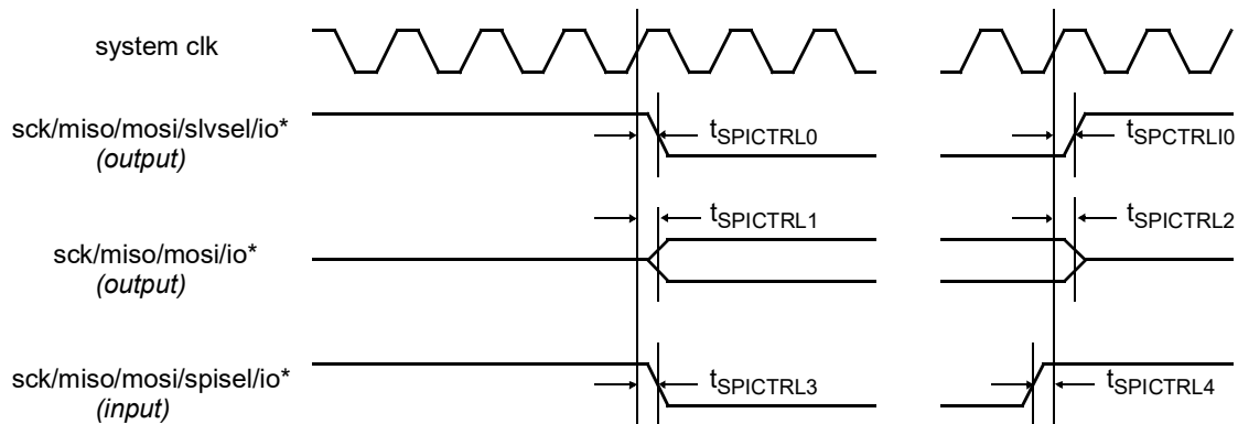
Figure 325. Timing waveforms
