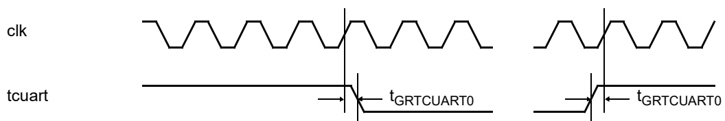
Figure 375. Timing waveforms
