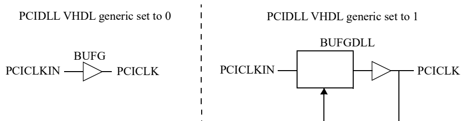
Figure 51. Virtex PCI clock generation
