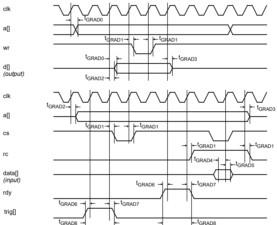
Figure 131. Timing waveforms
