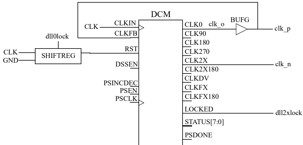
Figure 53. Virtex 2/4 generation of CLK2X clock when VHDL generic clk2xen is non-zero
