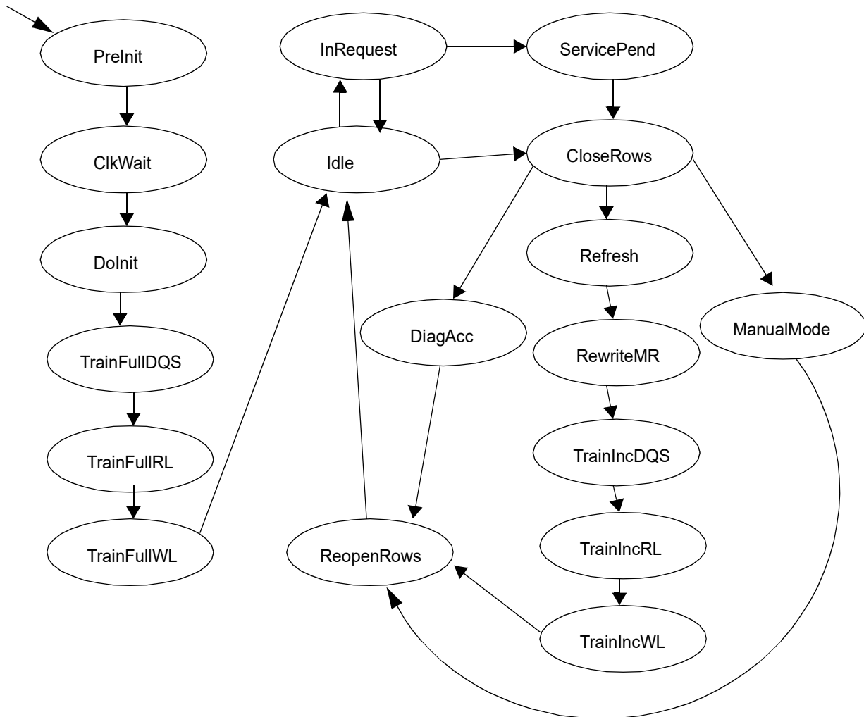
Figure 72. Simplified state diagram of DDR2/DDR3 controller back-end
