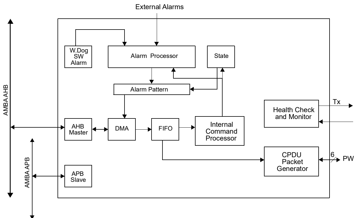
Figure 397. Block diagram
