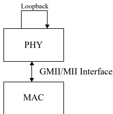
Figure 308. Block diagram of the PHY simulation model connected to a MAC.
