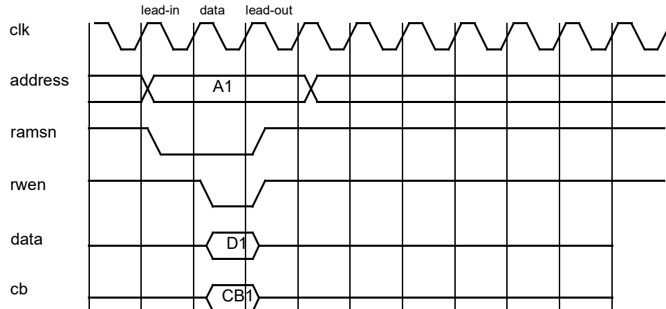
Figure 289. Sram write cycle (0-waitstates)
