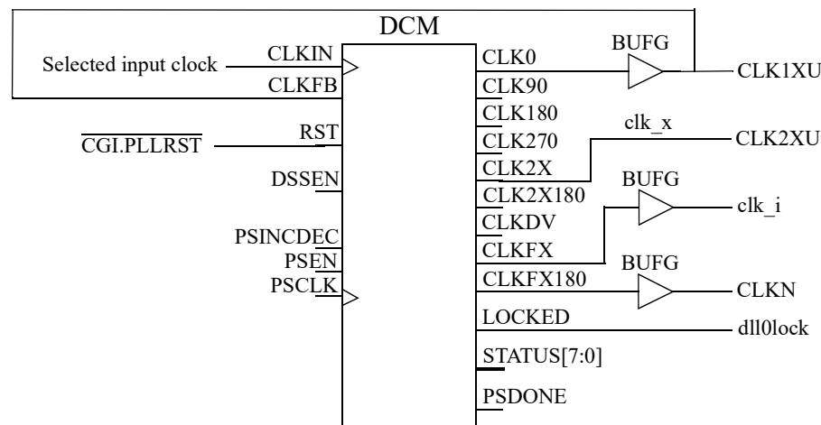
Figure 52. Virtex 2/4 generation of main clock
