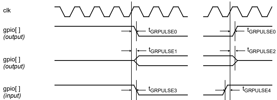
Figure 167. Timing waveforms
