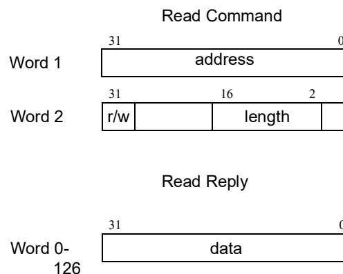
Figure 240. Layout of USB DCL read commands and replies.
