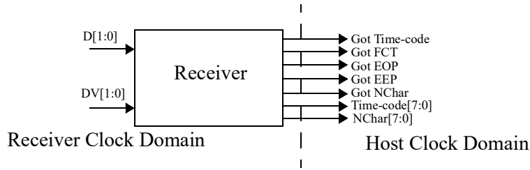
Figure 198. Schematic of the link interface receiver.
