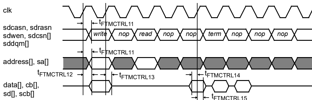
Figure 94. Timing waveforms - SDRAM accesses
