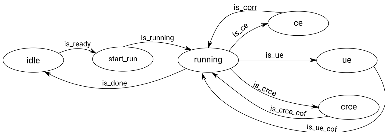
Figure 161. FSM of GRLSEDC IP
