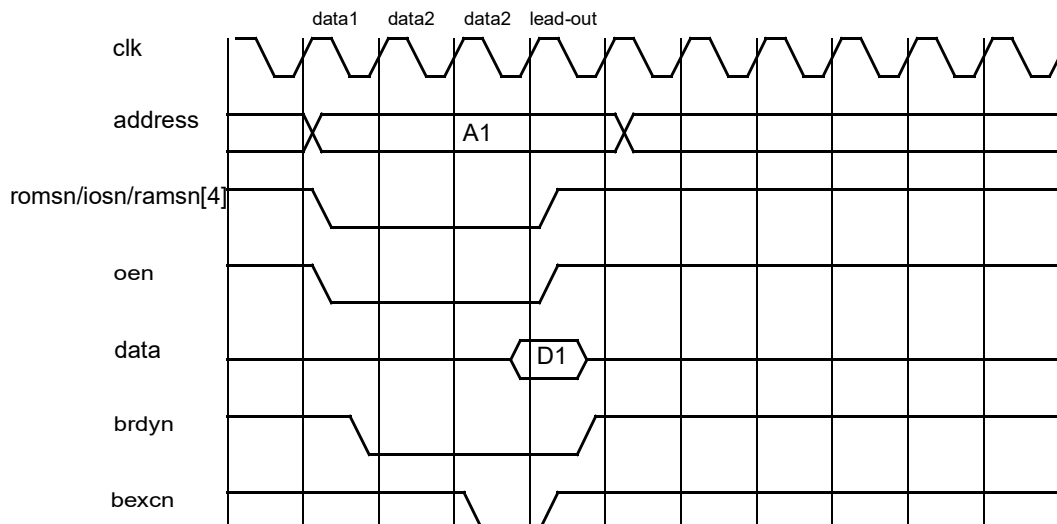
Figure 88. BRDYN (asynchronous) sampling and BEXCN timing. Lead-out cycle is only applicable for I/O-accesses.
