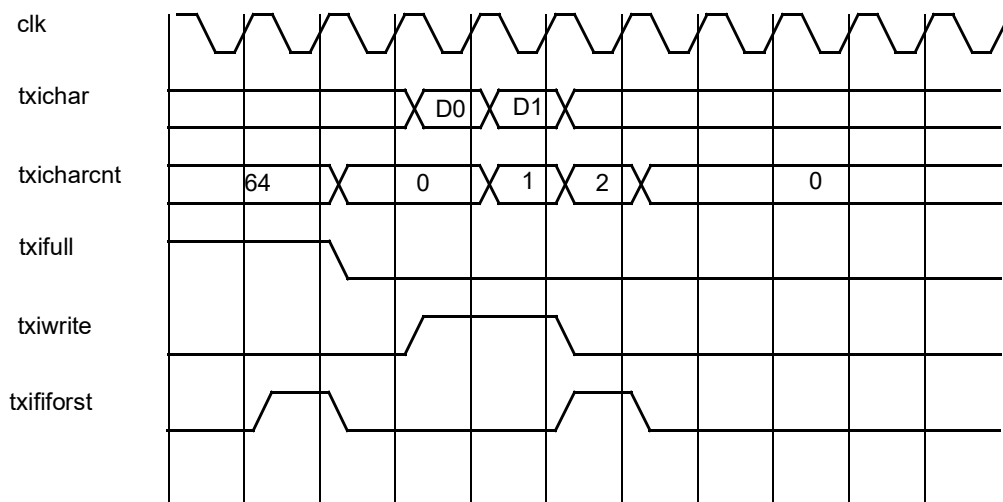
Figure 211. Use of txififorst.
