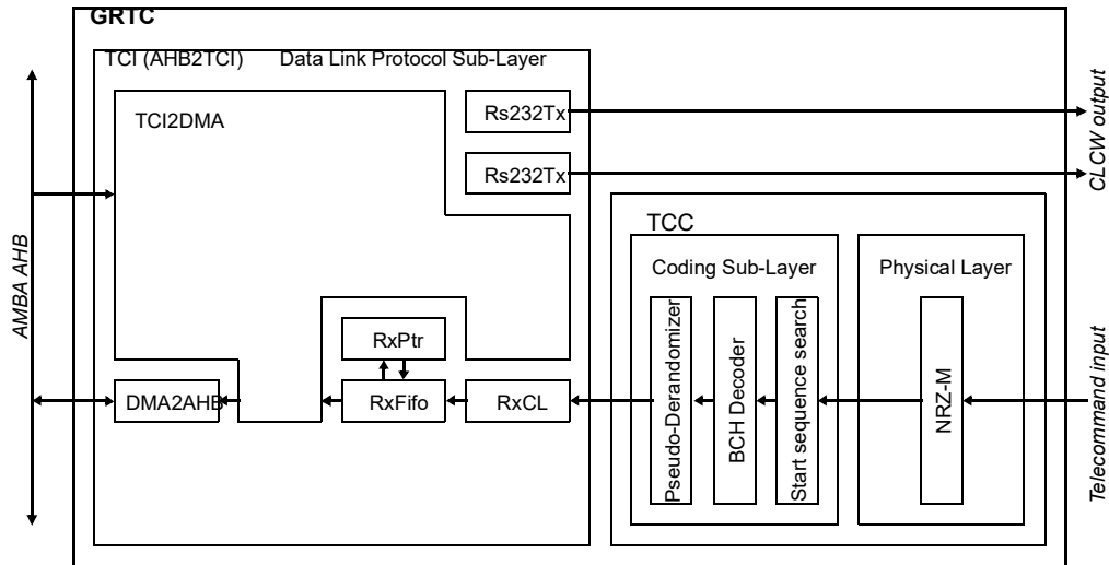
Figure 363. Detailed block diagram showing the internal structure
