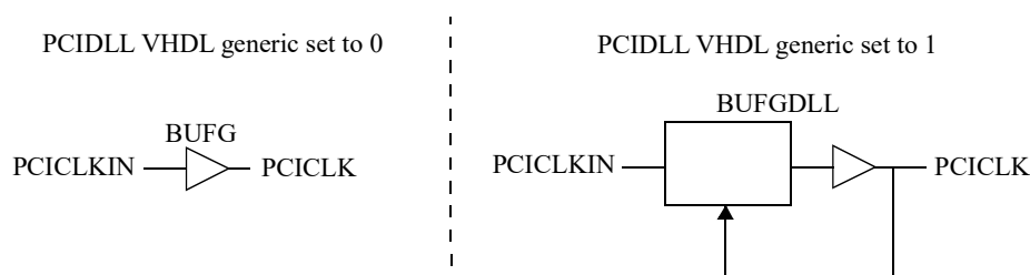
Figure 62. Virtex 5 PCI clock generation
