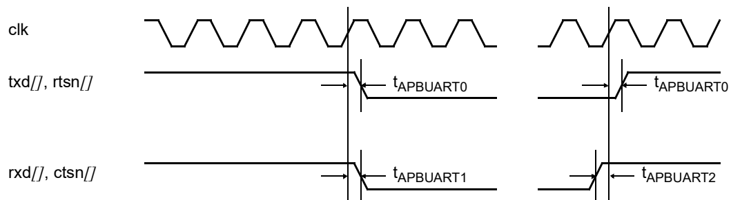
Figure 398. Timing waveforms
