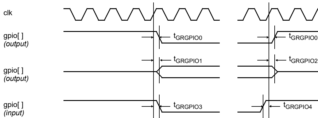
Figure 150. Timing waveforms
