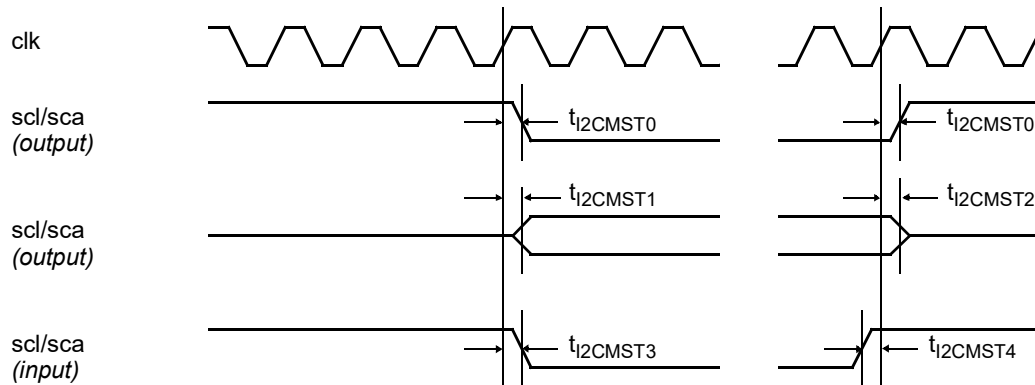
Figure 249. Timing waveforms
