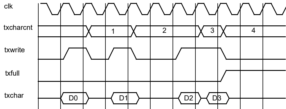
Figure 216. Transmitter FIFO interface write cycle.
