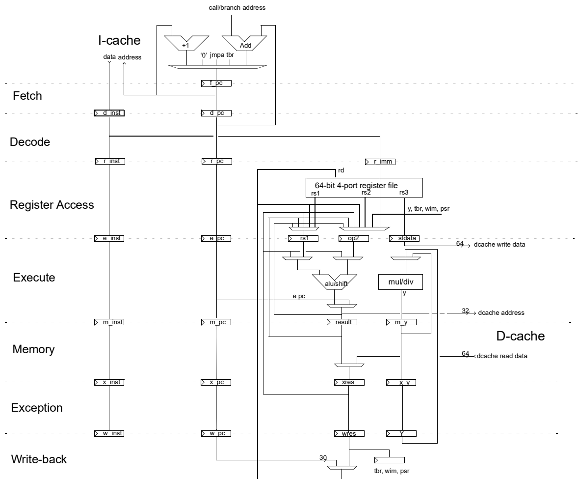
Figure 268. LEON4 integer unit datapath diagram
