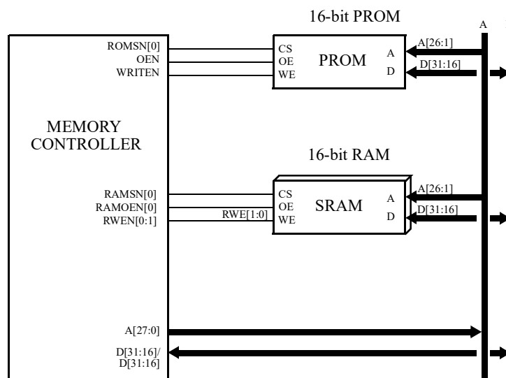
Figure 86. 16-bit memory interface example
