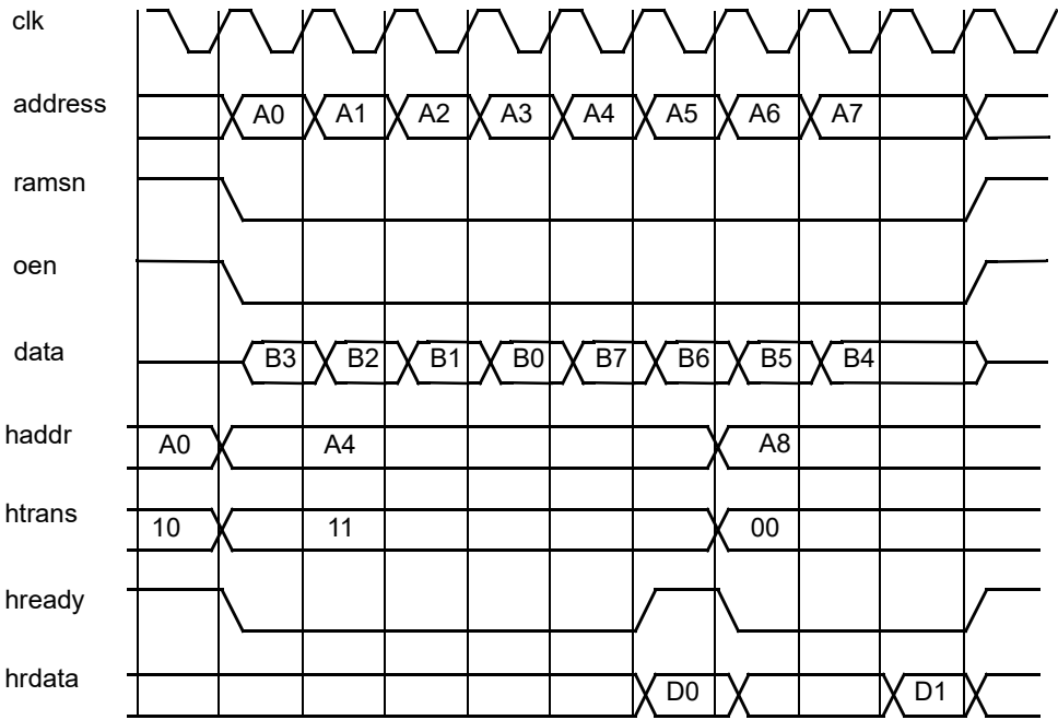
Figure 113. 32-bit SRAM sequential read accesses with 0 wait-states and EDAC enabled.
