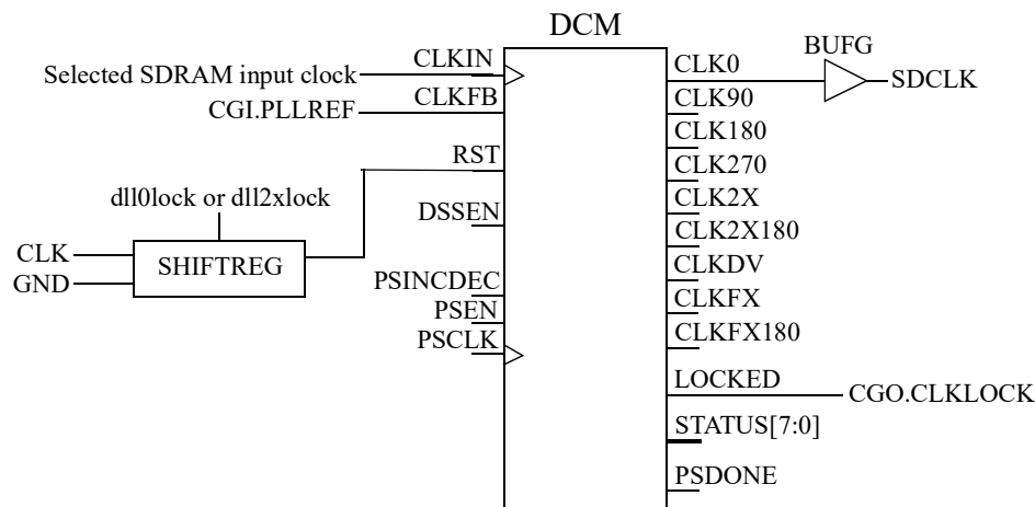
Figure 61. Virtex 5 generation of SDRAM clock
