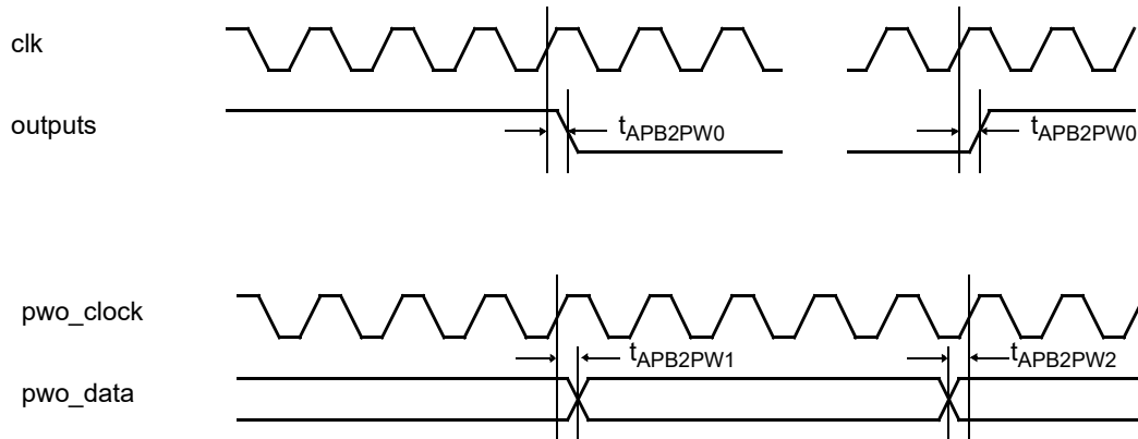
Figure 396. Timing waveforms
