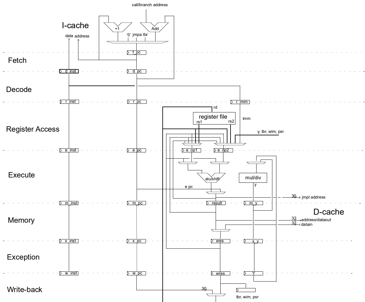
Figure 259. LEON3 integer unit datapath diagram
