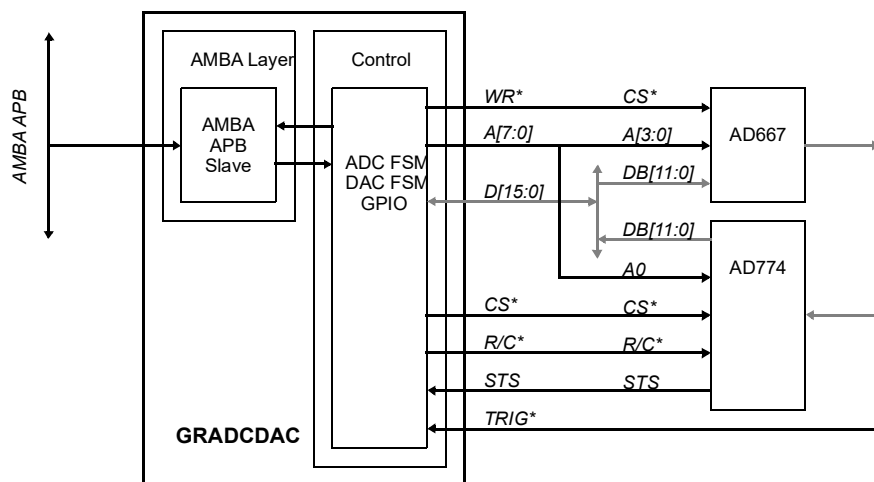
Figure 128. Block diagram and usage example
