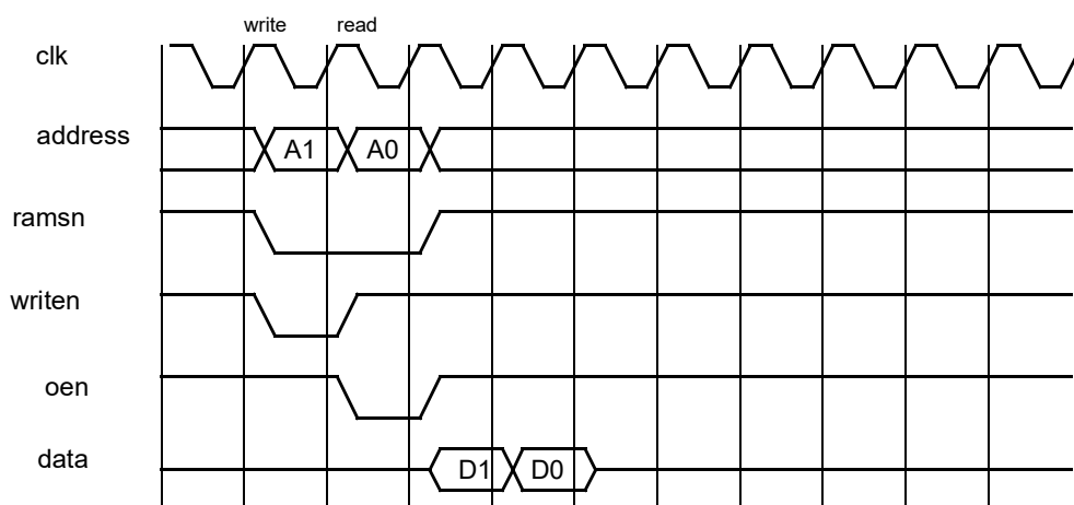
Figure 337. 32-bit SSRAM write cycle
