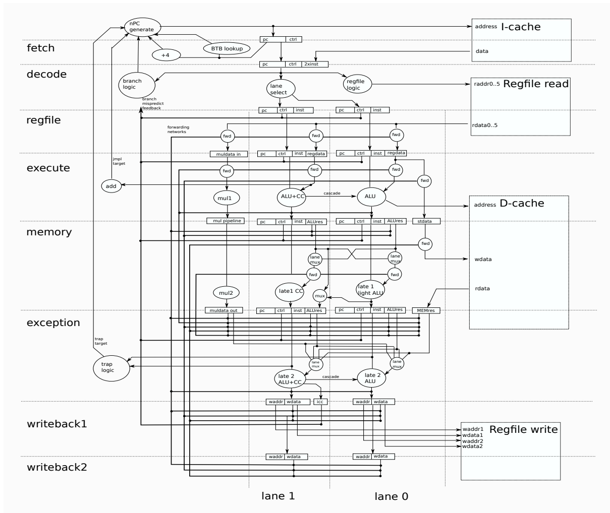
Figure 275. LEON5 integer unit datapath diagram
