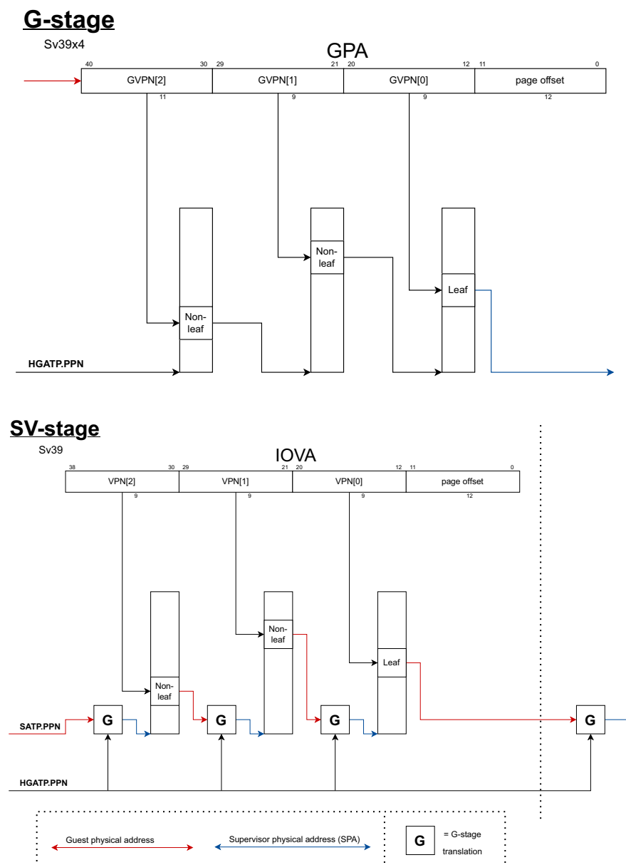
Figure 158. RISC-V two-stage address translation using Sv39
