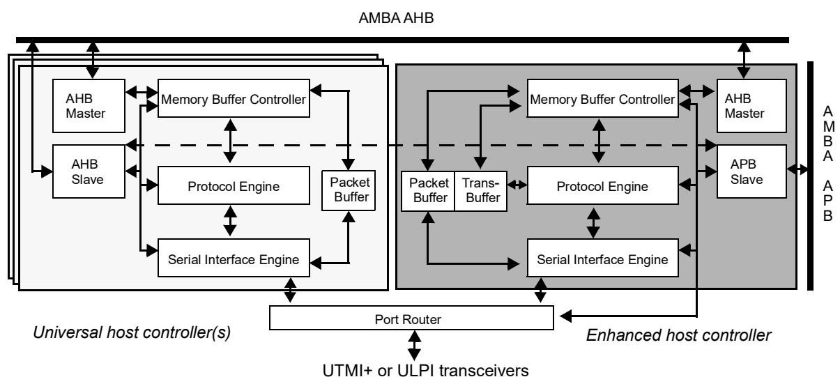
Figure 242. Block diagram of both host controller types
