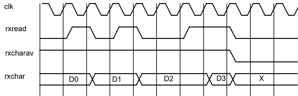
Figure 217. Receiver FIFO interface read cycle.
