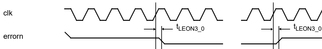
Figure 273. Timing waveforms
