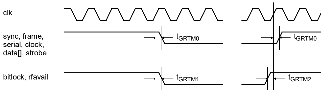
Figure 353. Timing waveforms
