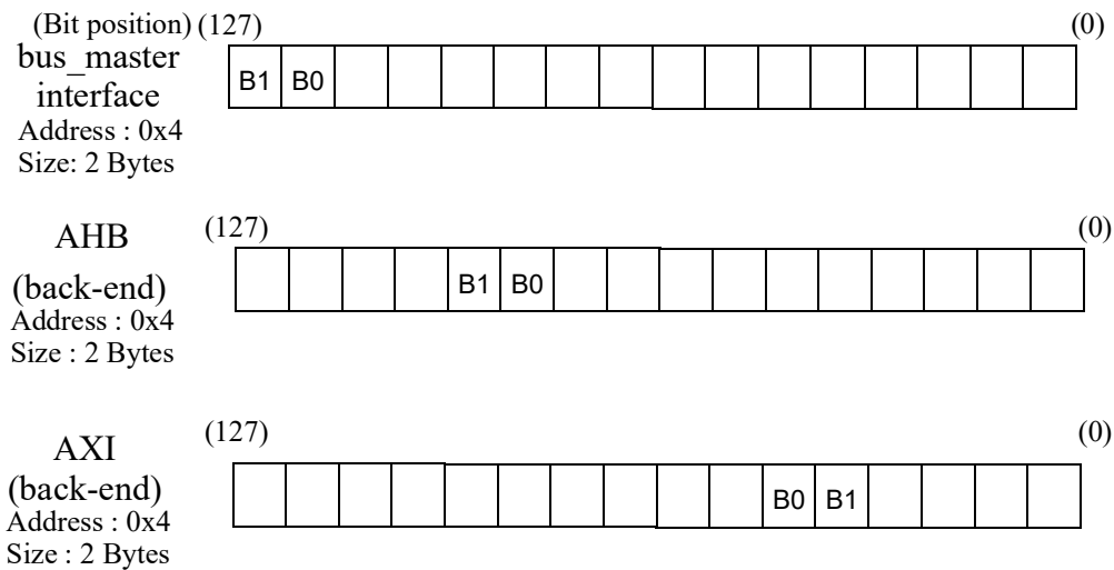
Figure 229. 2 Byte Access on AHB and AXI back-ends (BM_DW=128-bit, BE_DW=128-bit)
