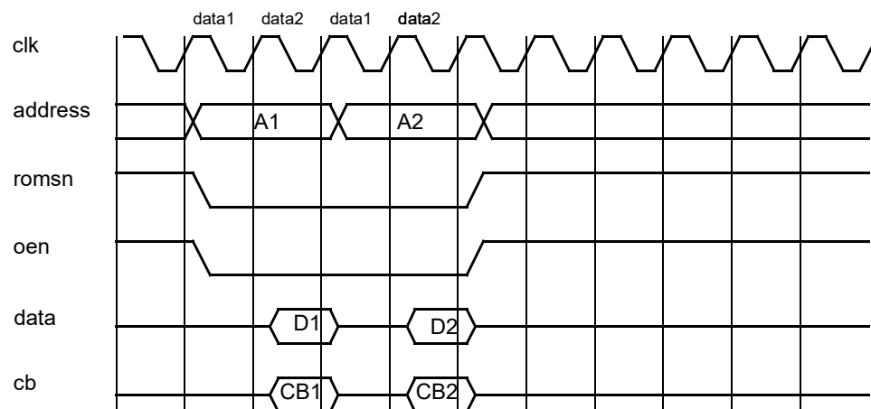
Figure 76. Prom consecutive read cycles.
