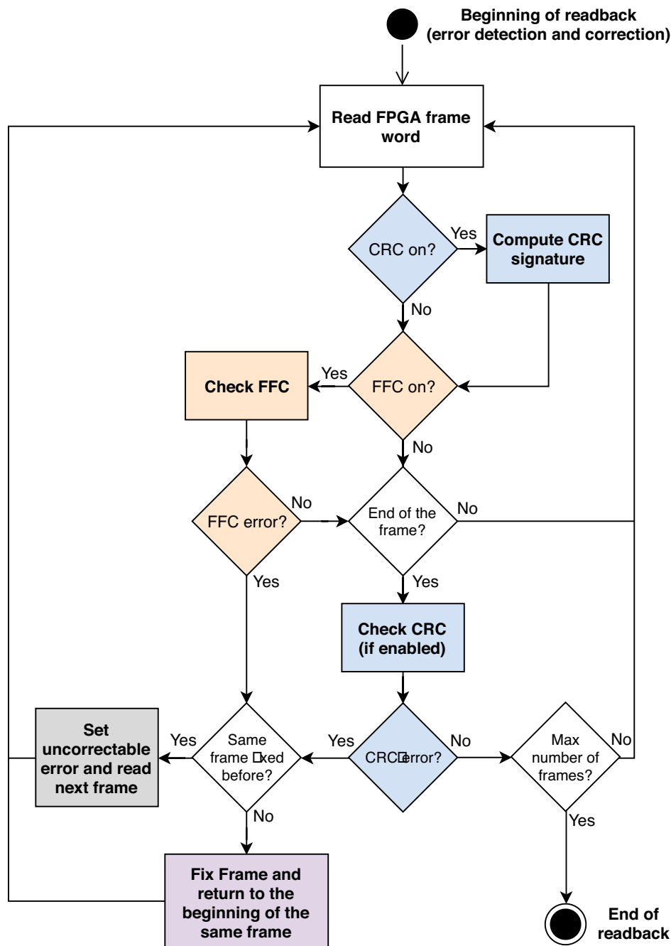
Figure 174. GRSCRUB flow in readback scrubbing mode for error detection and correction
