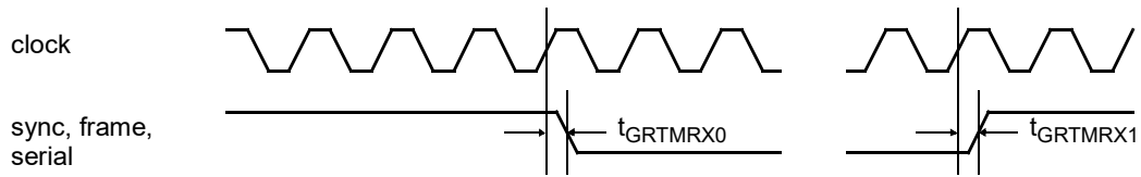
Figure 359. Timing waveforms
