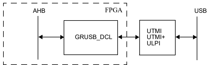
Figure 236. USBDC connected to an external UTM.
