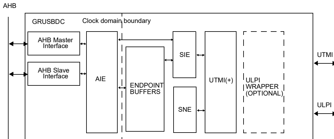
Figure 234. Block diagram of the internal structure of the core.
