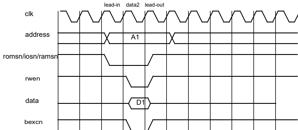
Figure 295. Write cycle with BEXCN. Chip-select (iosn) is not asserted in lead-in cycle for io-accesses.
