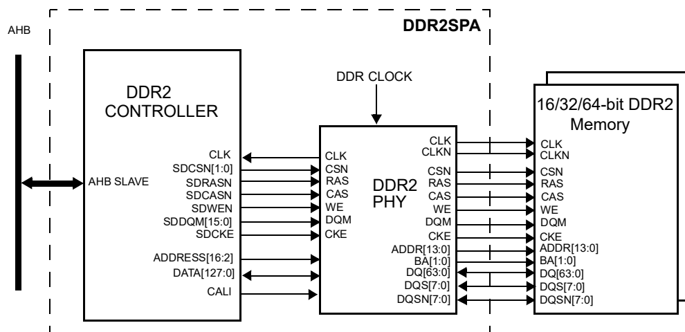
Figure 66. DDR2SPA Memory controller connected to AMBA bus and DDR2 SDRAM
