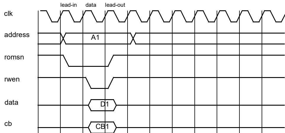
Figure 284. Prom write cycle (0-waitstates)
