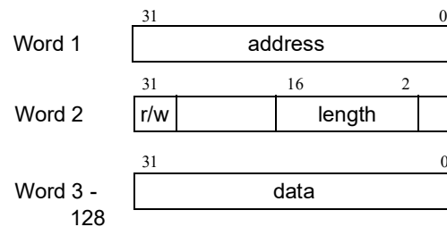
Figure 239. Layout of USB DCL write commands.
