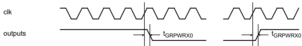
Figure 387. Timing waveforms
