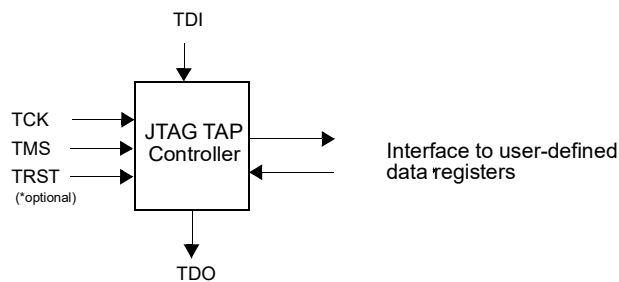
Figure 346. TAP controller block diagram
