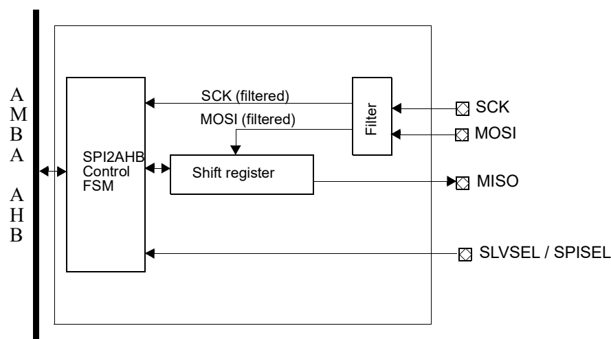
Figure 321. Block diagram, optional APB interface not shown
