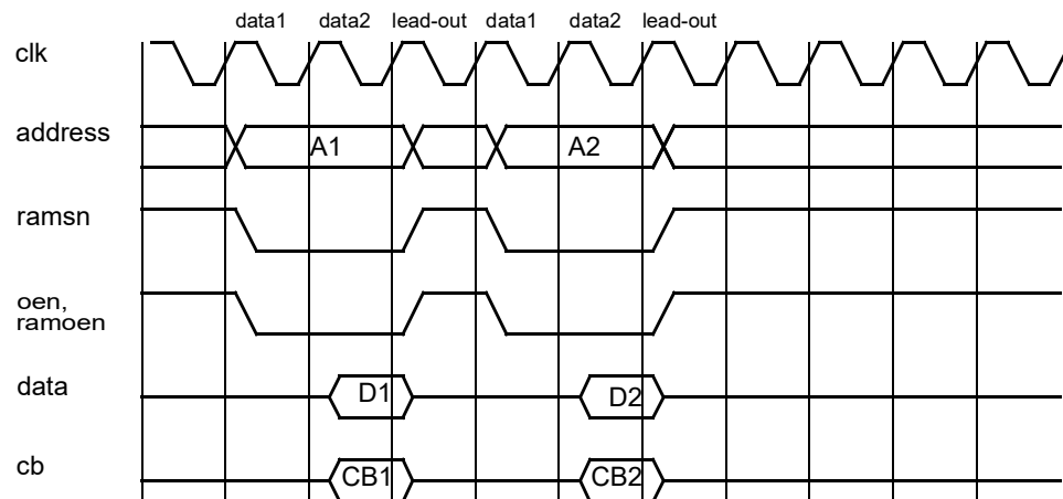
Figure 288. SRAM non-consecutive read cycles.
