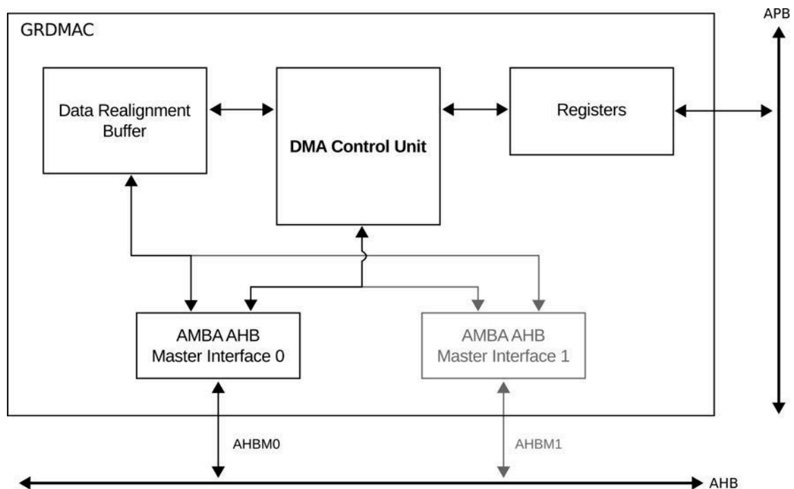
Figure 138. Block diagram
