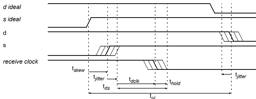
Figure 194. Skew and jitter timing waveforms
