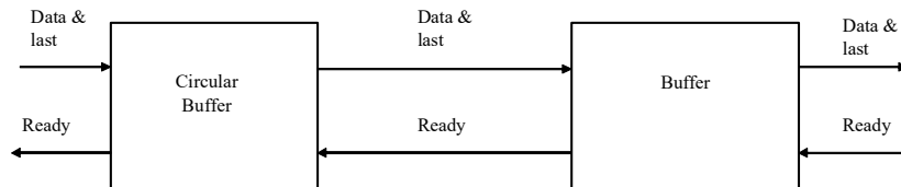
Figure 36. Figure: AXI4-S gearbox architecture
