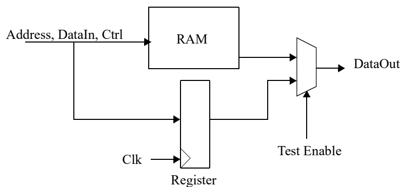
Figure 344. Scan test support
