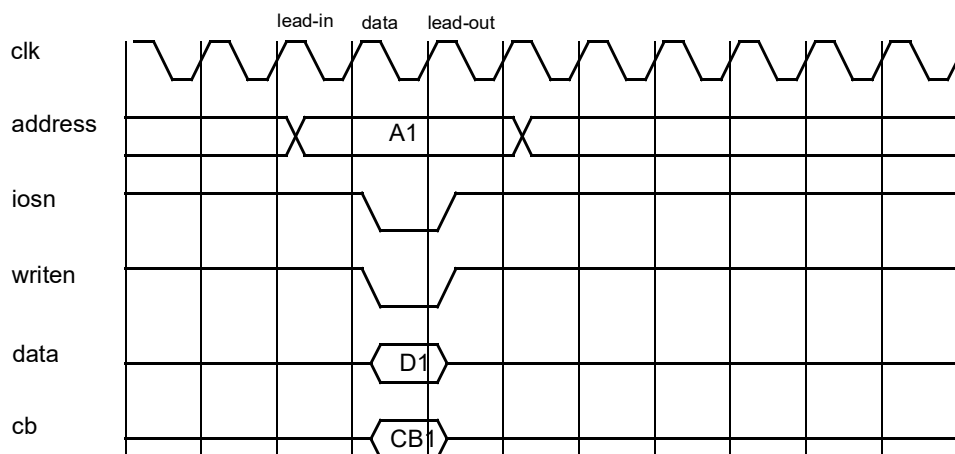
Figure 81. I/O write cycle (0-waitstates)
