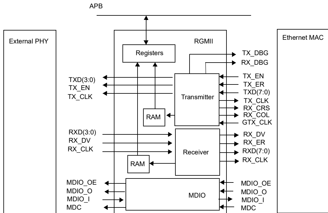
Figure 309. Block diagram of the internal structure of the RGMII.
