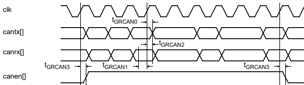
Figure 134. Timing waveforms
