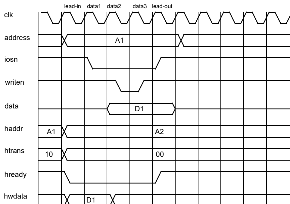
Figure 108. I/O write access with 0 wait-states.
