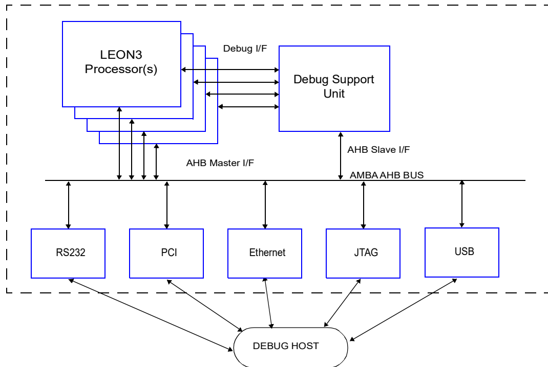
Figure 67. LEON3/DSU Connection
