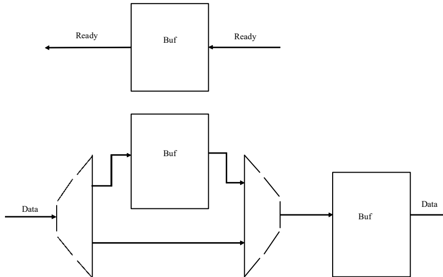
Figure 35. Figure: AXI-S buffer architecture
