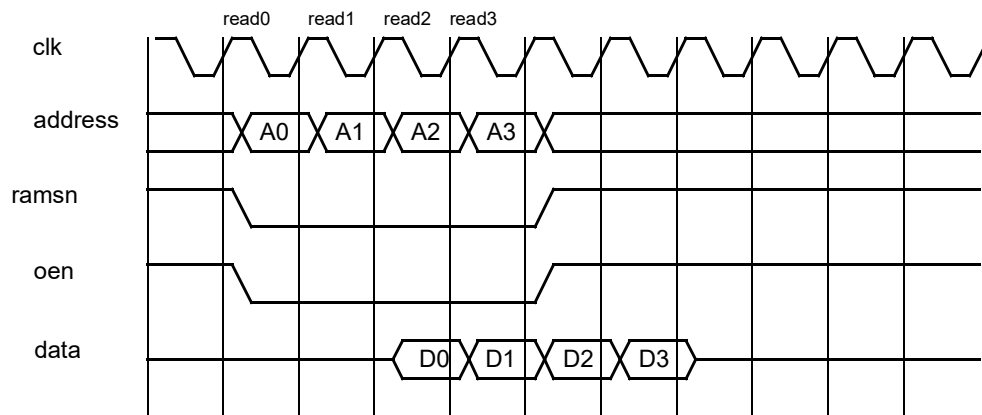
Figure 336. 32-bit SSRAM read cycle
