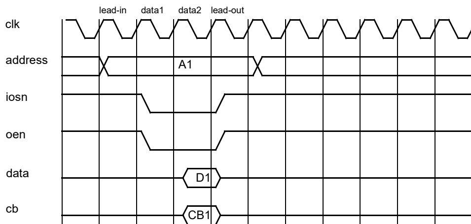
Figure 80. I/O read cycle (0-waitstates)
