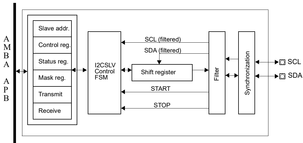
Figure 250. Block diagram
