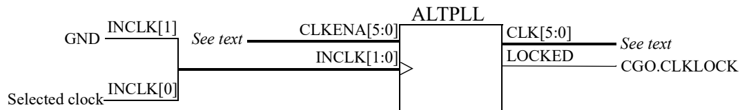
Figure 40. Altera Cyclone III ALTPLL
