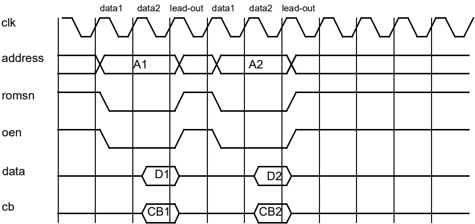
Figure 281. Prom non-consecutive read cycles.
