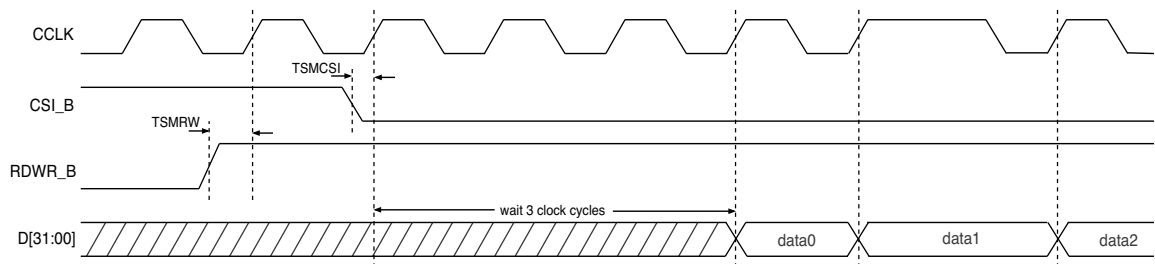
Figure 177. SelectMap timing characteristics for data reading from FPGA
