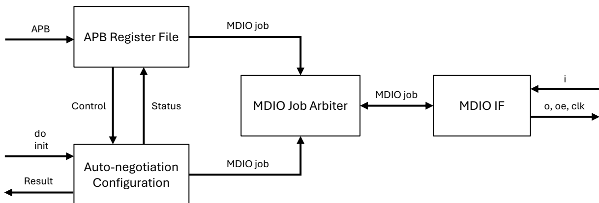
Figure 296. MDIO_CTRL block diagram
