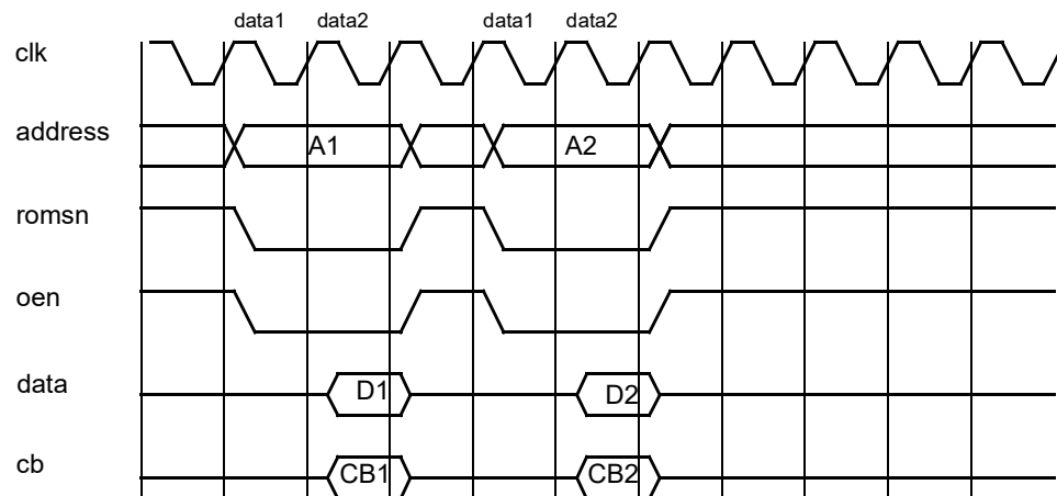
Figure 75. Prom non-consecutive read cycles.
