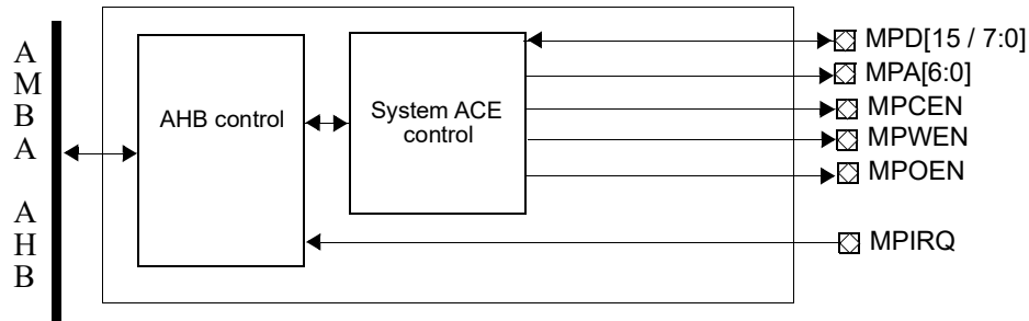
Figure 127. Block diagram
