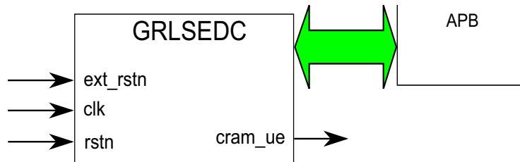
Figure 159. Top-level view of GRLSEDC IP.
