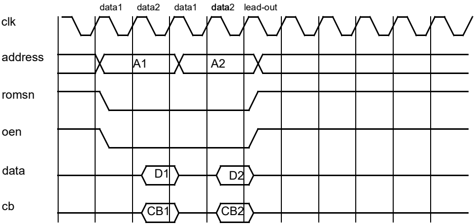
Figure 282. Prom consecutive read cycles.
