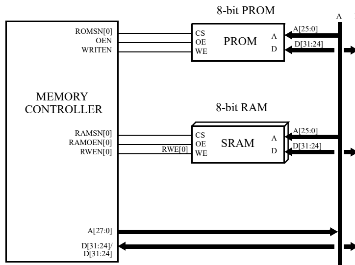
Figure 85. 8-bit memory interface example
