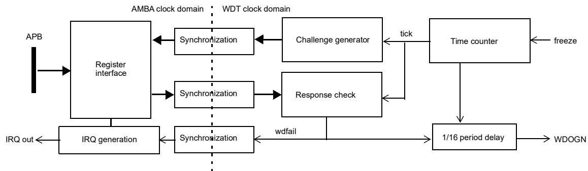
Figure 243. Functional block diagram of GRWATCHDOG
