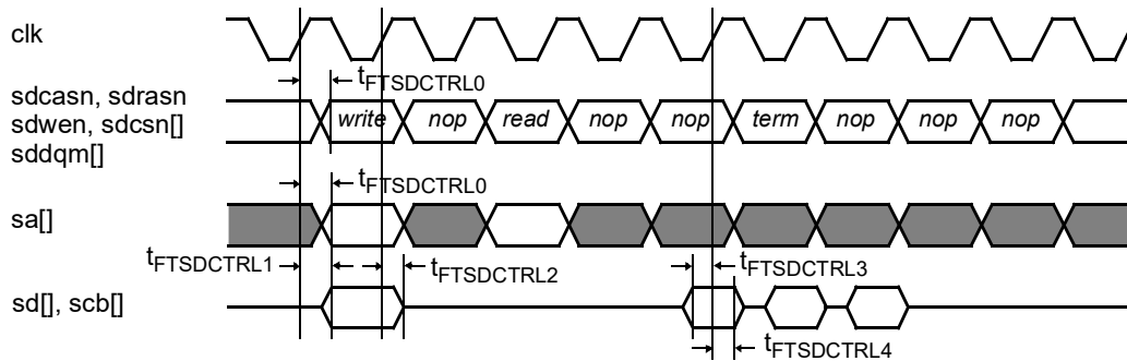
Figure 96. Timing waveforms
