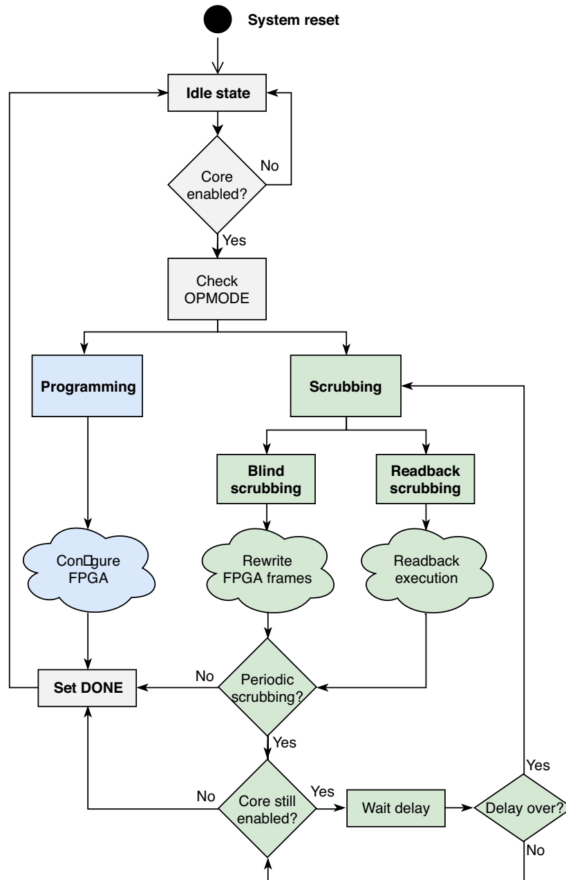
Figure 173. GRSCRUB flow for programming and scrubbing operation modes
