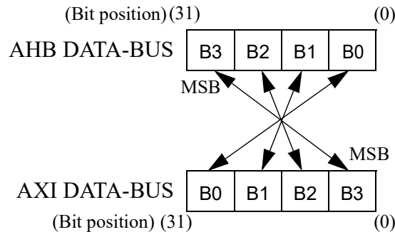
Figure 4. Big-endian AHB to byte-invariant Big-endian AXI translation (32-bit data-width)
