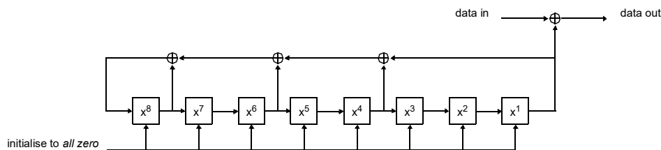
Figure 348. Pseudo-randomiser
