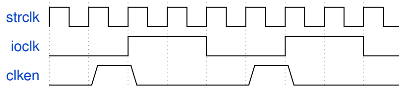
Figure 156. Expected clken input behavior when using a 4:1 relationship between strclk and ioclk
