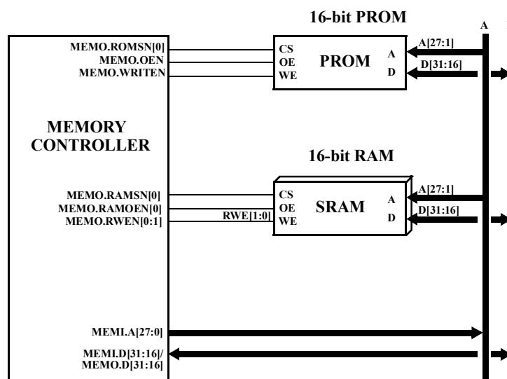
Figure 291. 16-bit memory interface example
