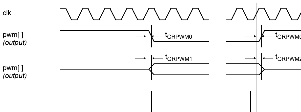
Figure 168. Timing waveforms
