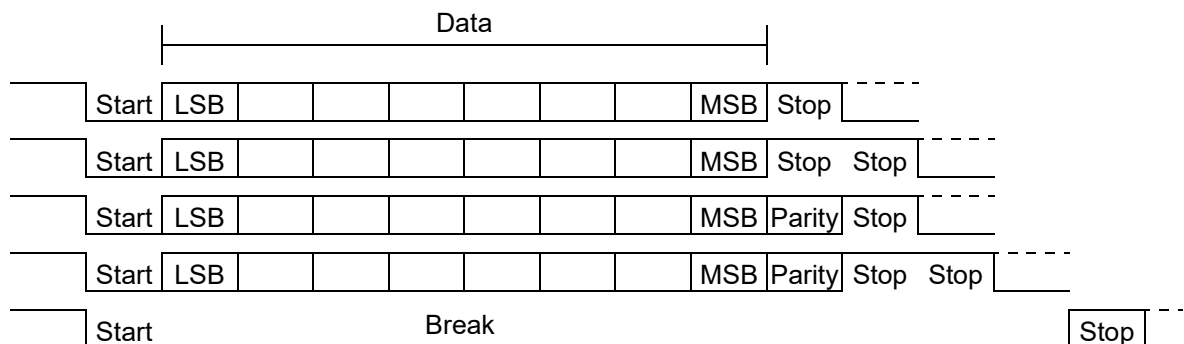
Figure 356. Asynchronous bit serial protocol / waveform
