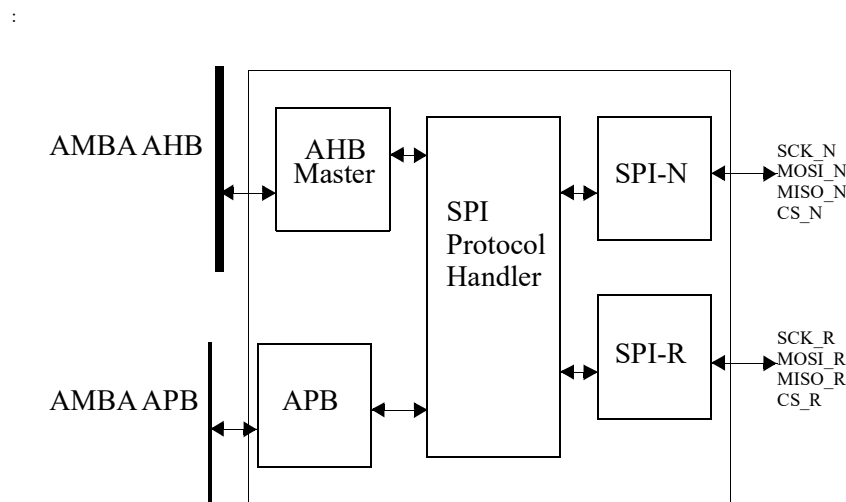
Figure 329. Block diagram
