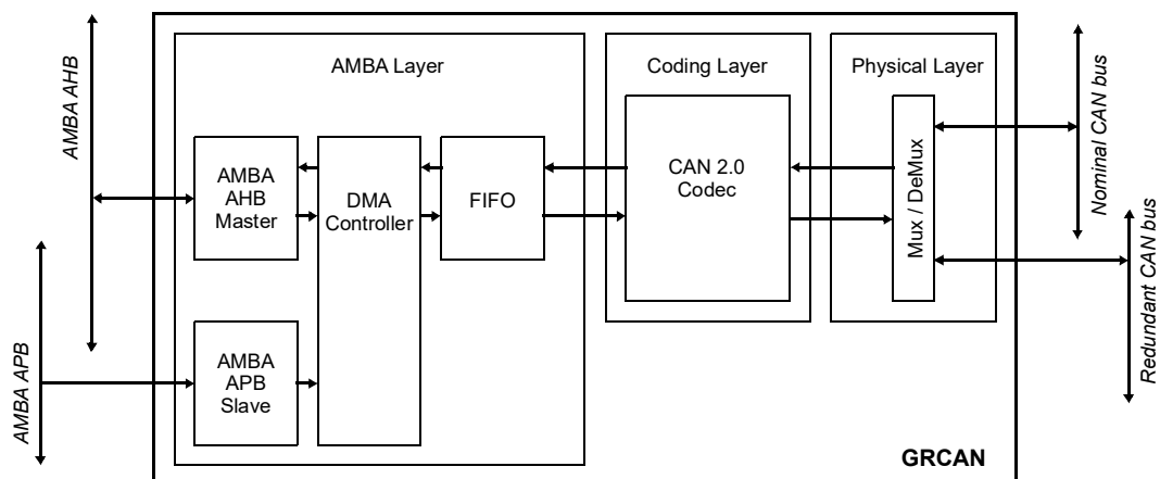
Figure 133. Block diagram
