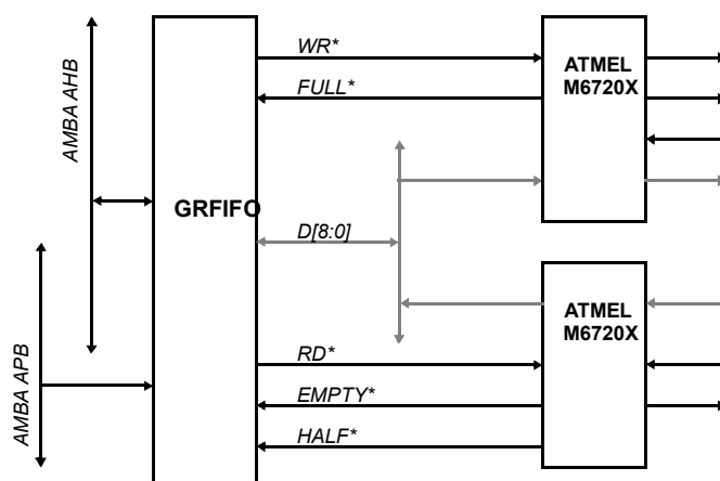
Figure 143. Example of usage, with shared external data bus
