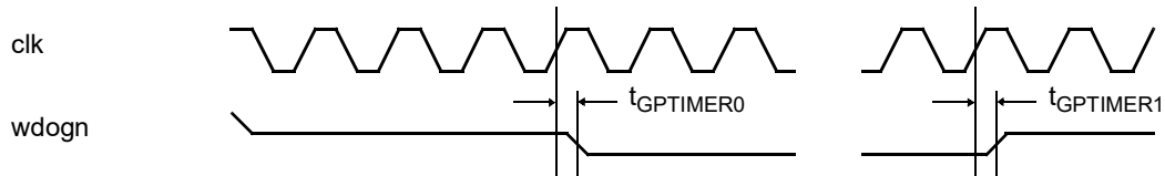
Figure 121. Timing waveforms
