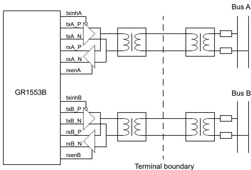
Figure 122. Interface between core and MIL-STD-1553B bus (dual-redundant, transformer coupled)
