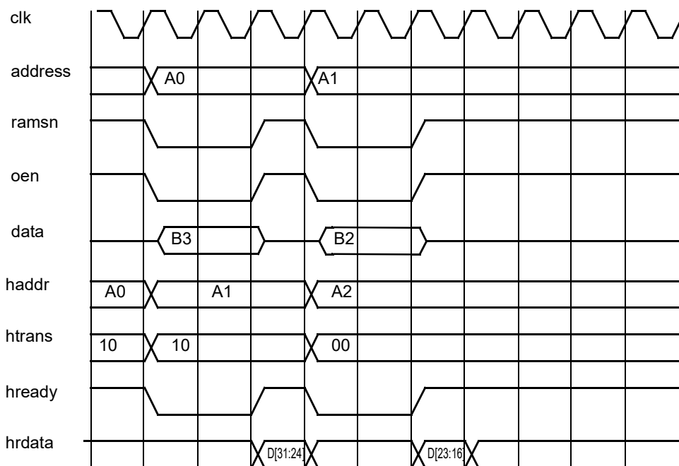
Figure 116. 8-bit SRAM non-sequential read access with 0 wait-states and EDAC enabled.
