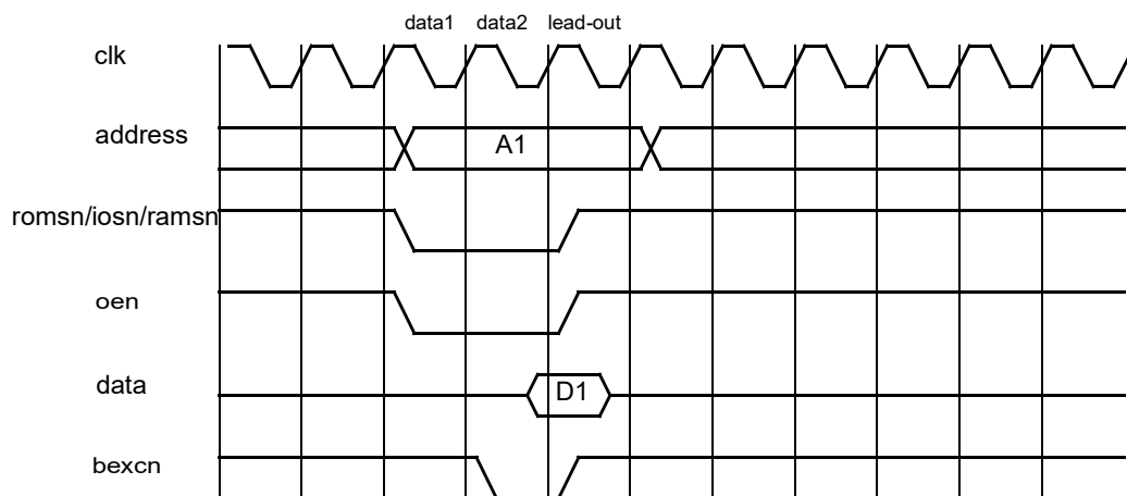
Figure 294. Read cycle with BEXCN.
