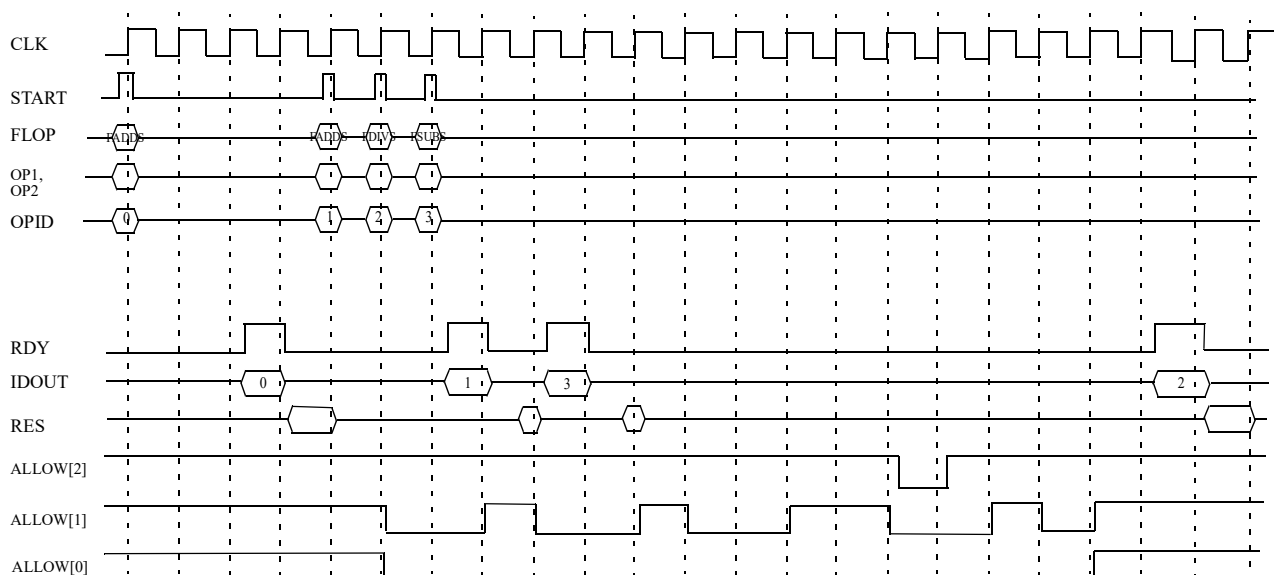
Figure 148. Signal timing
