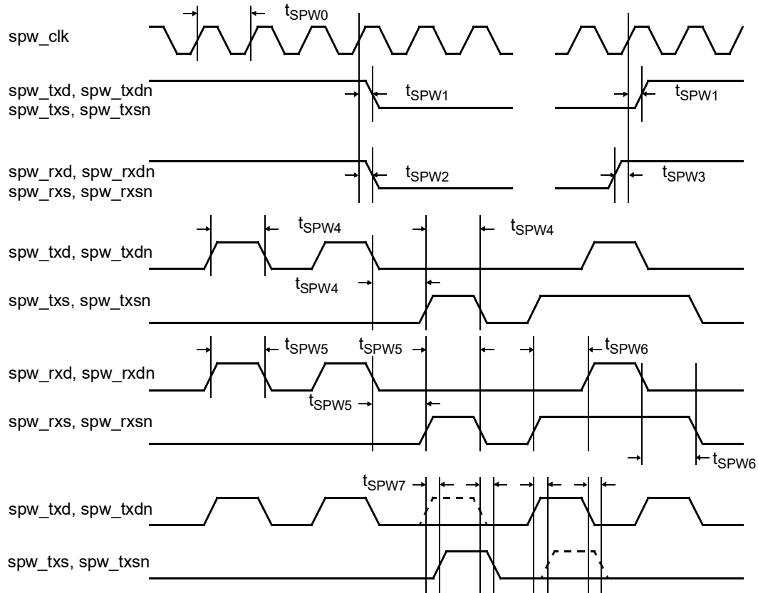
Figure 223. Timing waveforms
