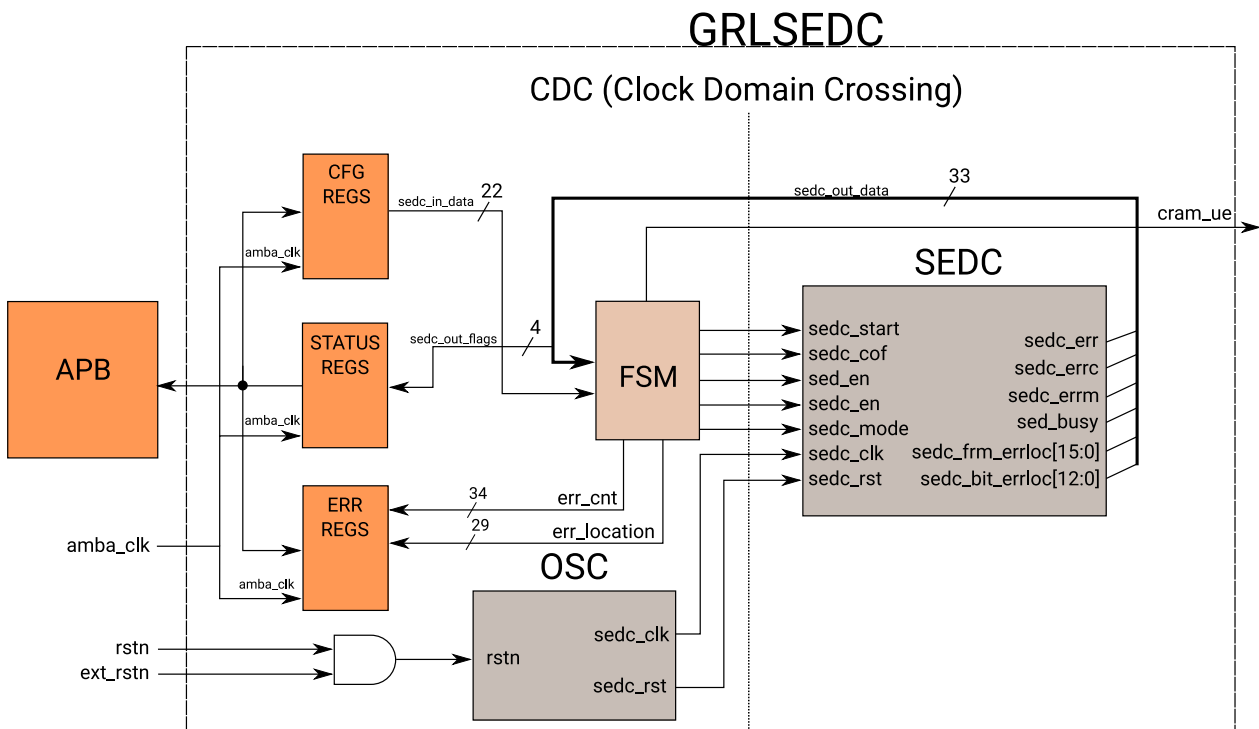
Figure 160. Internal view of GRLSEDC IP.
