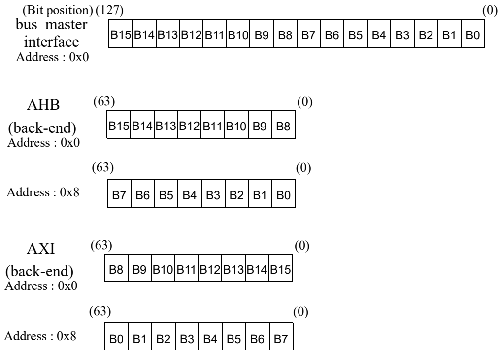
Figure 228. 16 Byte Access on AHB and AXI back-ends (BM_DW=128-bit, BE_DW=64-bit)
