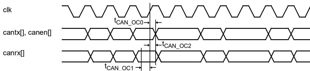
Figure 38. Timing waveforms
