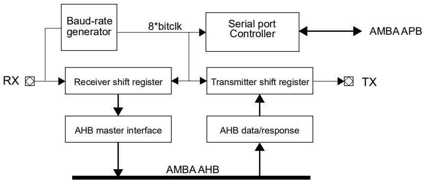
Figure 8. Block diagram
