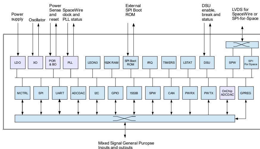
Figure 8. Architectural block diagram showing connections to the I/O switch matrix
