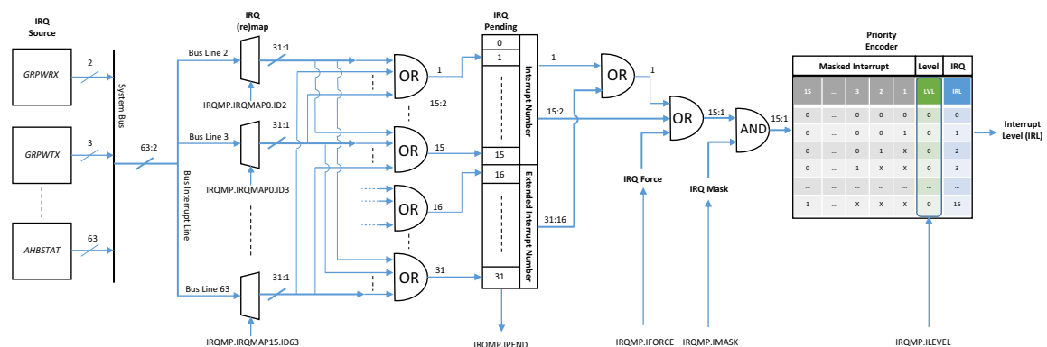
Figure 71. System and Interrupt controller block diagram
