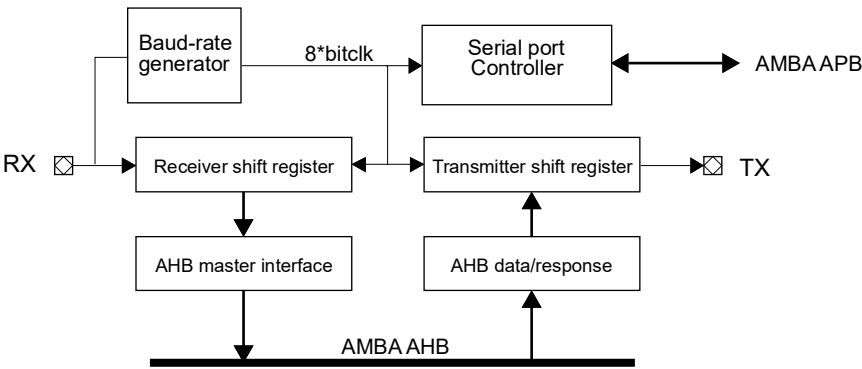
Figure 90. Block diagram
