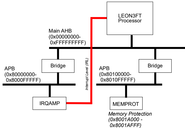
Figure 70. GR716A Interrupt controller bus connection
