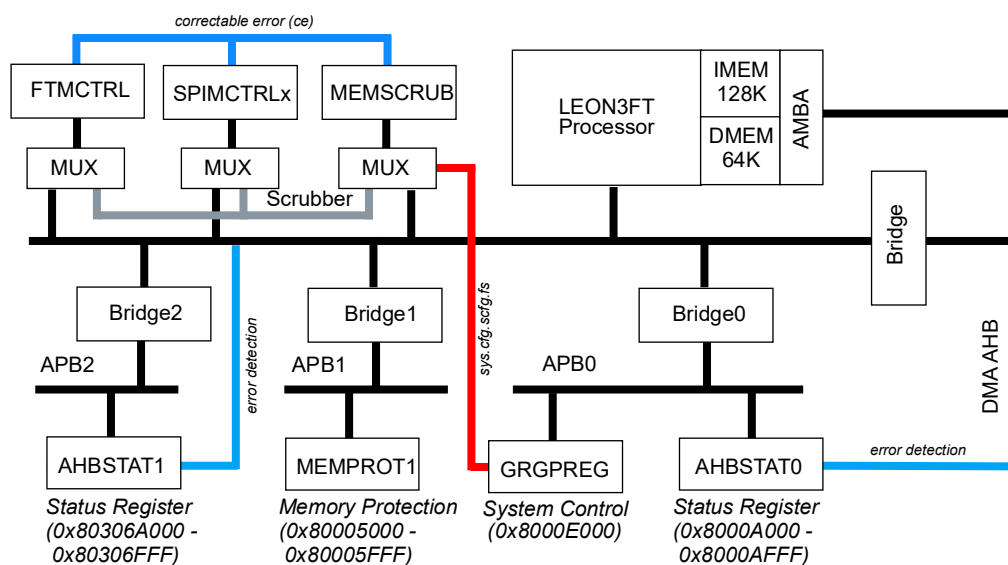
Figure 72. GR716A Scrubber and Status bus connection
