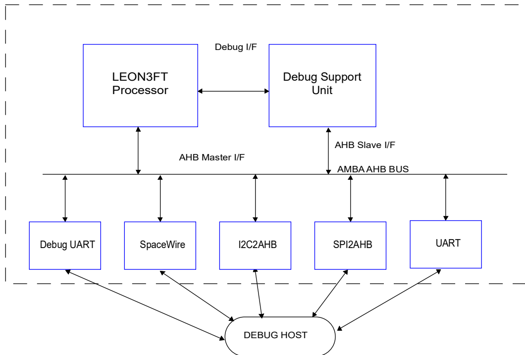
Figure 20. LEON3FT/DSU Connection
