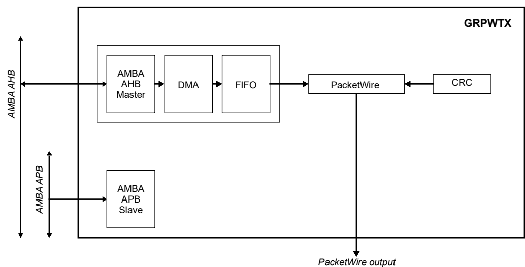
Figure 50. Block diagram
