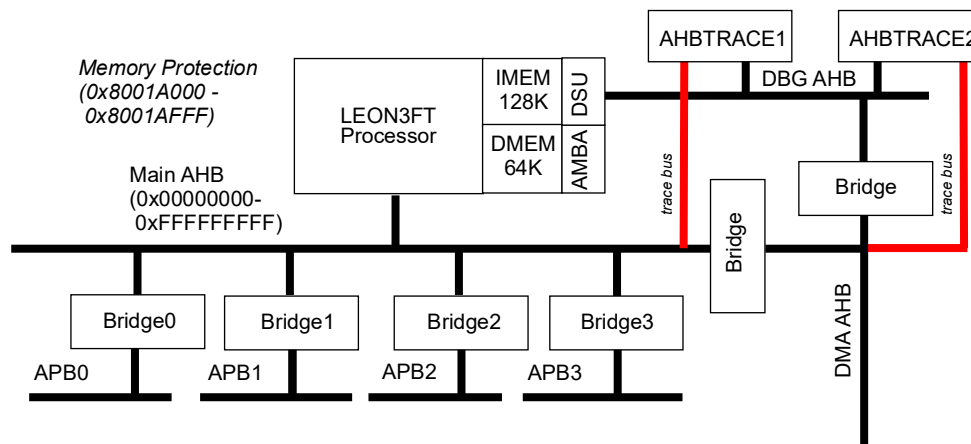
Figure 94. GR716A AHBTRACEx bus and pin connection
