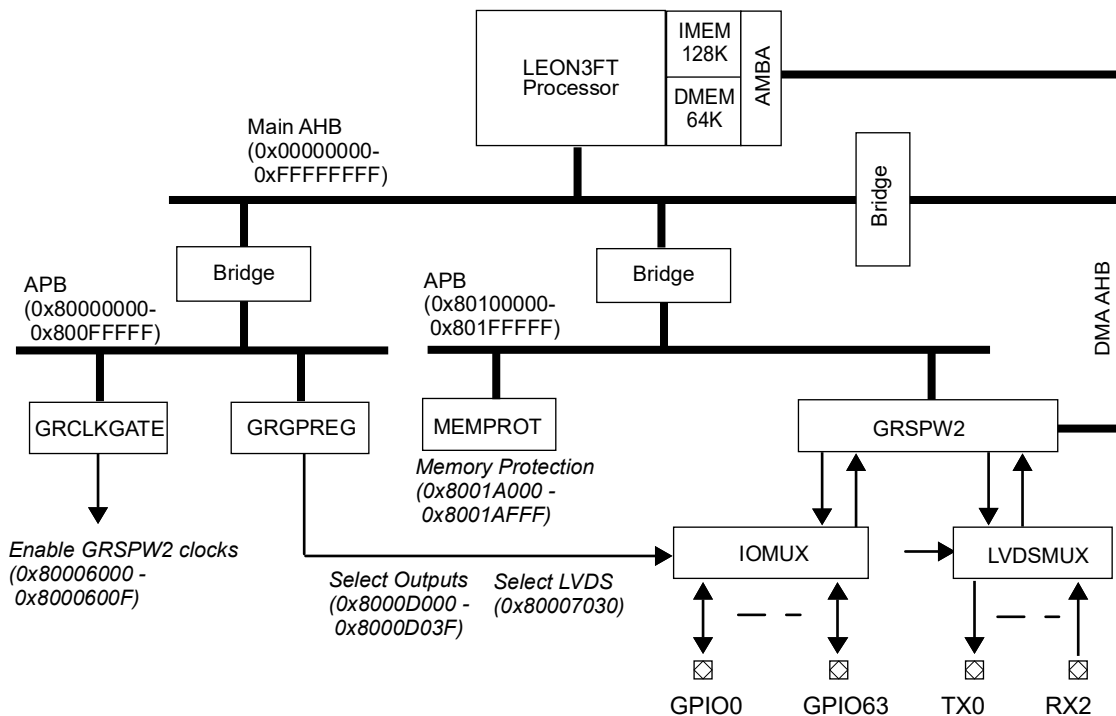
Figure 52. GR716A GRSPW2 bus and pin
