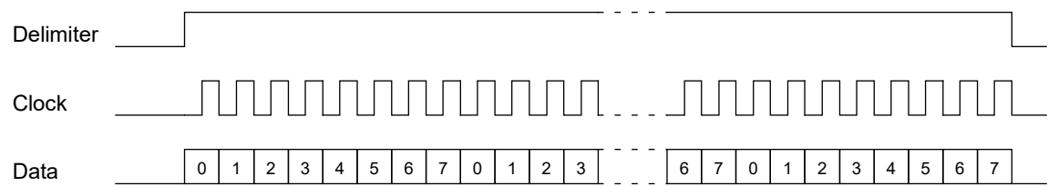
Figure 51. Synchronous bit serial waveform
