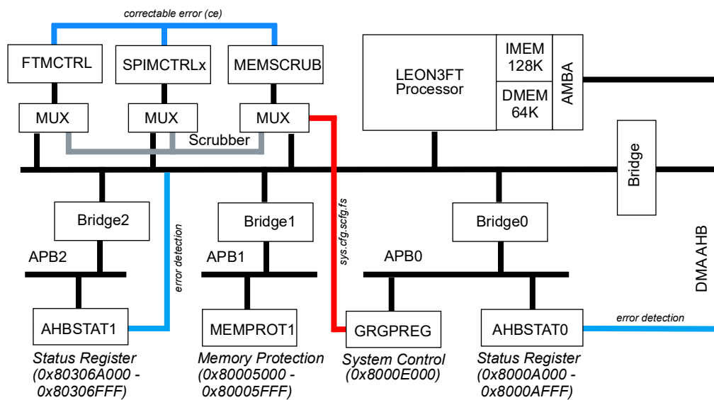
Figure 93. GR716A Status Register bus connection
