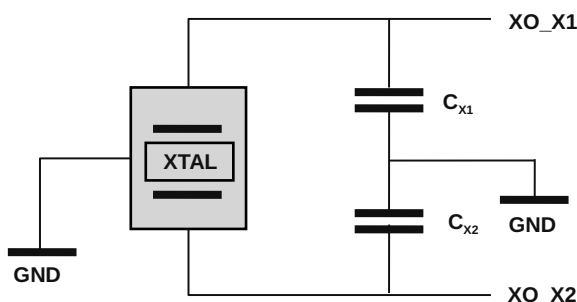
Figure 11. Connection diagram for C_{X1} and C_{X2} on PCB, where XO_X1 and XO_X2 are the XO connections on GR716A.
