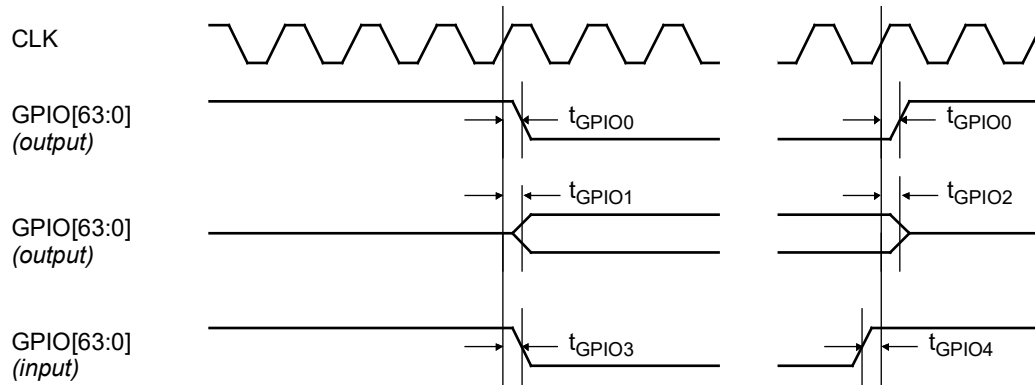
Figure 122. General purpose I/O timing waveforms
