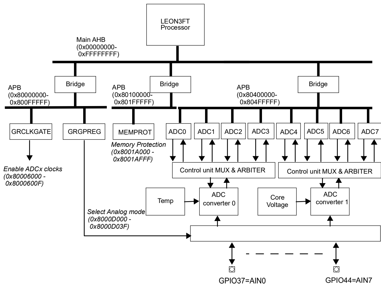
Figure 12. GR716A on-chip ADC bus and pin connections.
