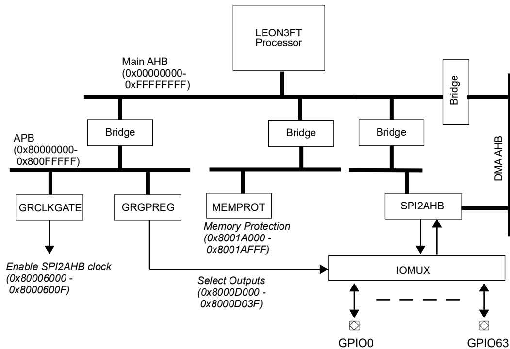
Figure 74. GR716A SPI2AHB bus and pin
