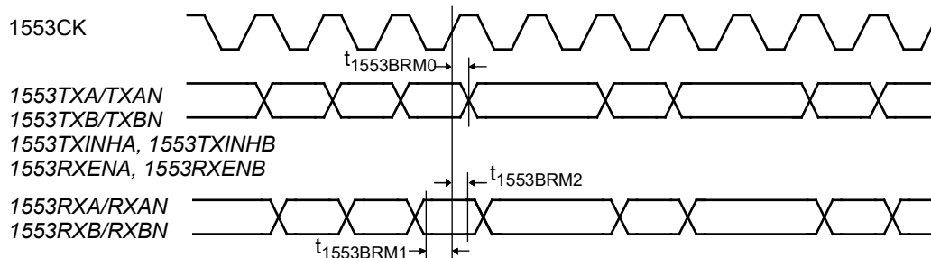
Figure 115. MIL-1553B timing waveforms
