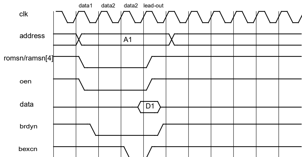
Figure 31. BRDYN (asynchronous) sampling and BEXCN timing.
