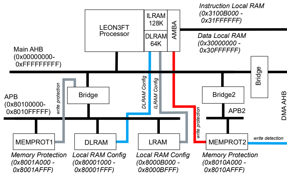
Figure 21. GR716A LRAM bus connection
