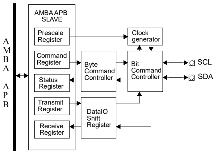
Figure 65. Block diagram
