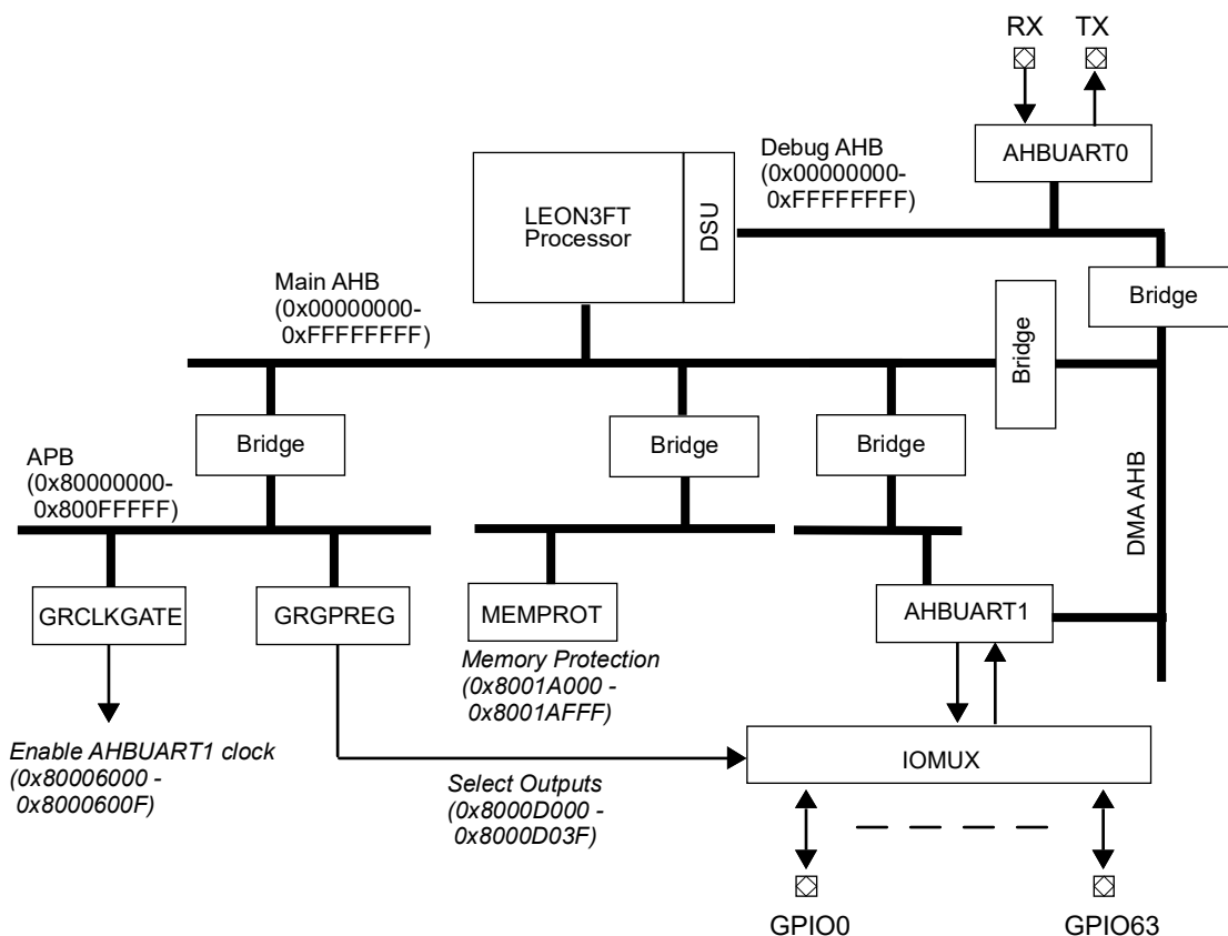
Figure 89. GR716A AHBUARTx bus and pin connection
