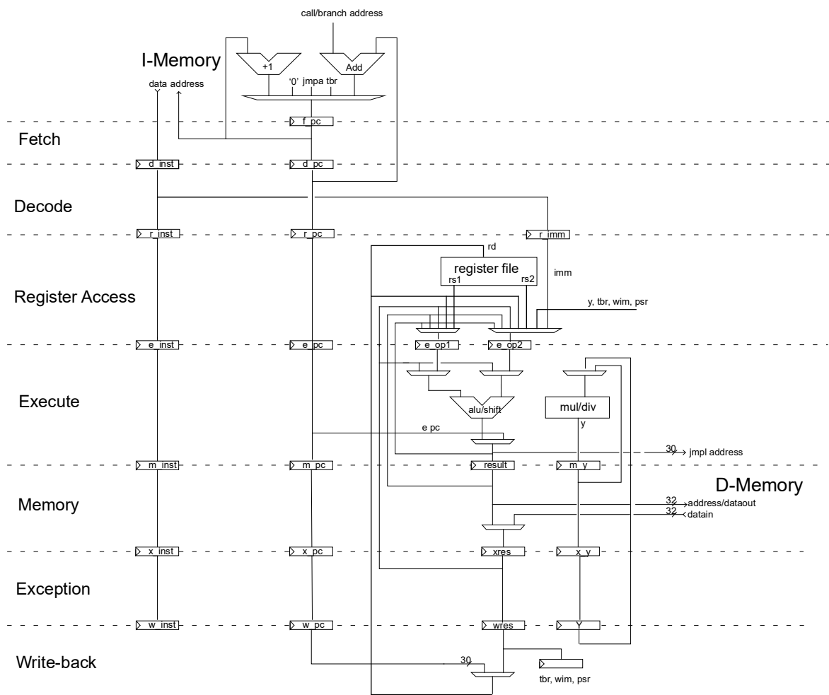
Figure 15. LEON3 integer unit datapath diagram
