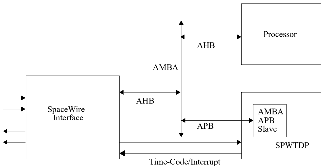
Figure 58. Block diagram
