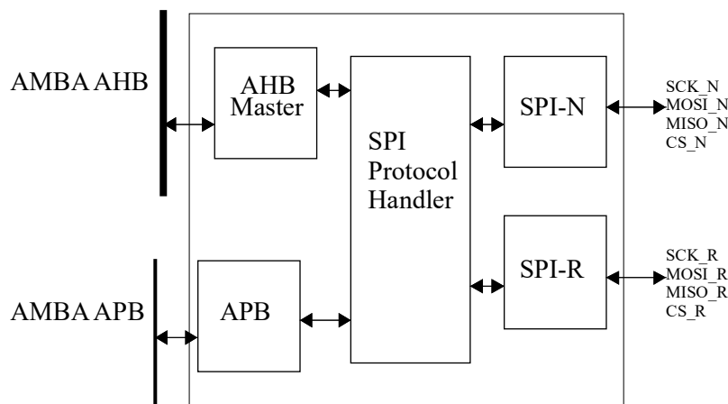
Figure 81. Block diagram
