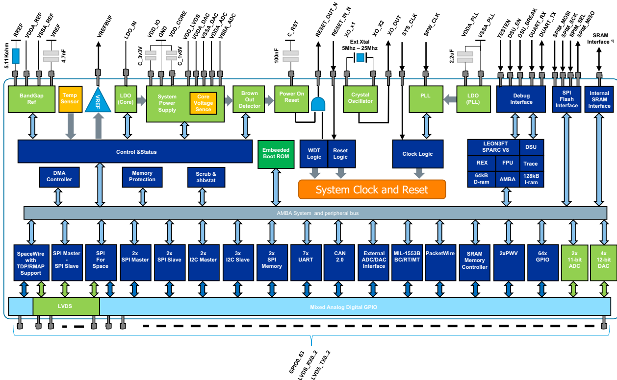
Figure 4. GR716A simplified block diagram of the analog/mixed and power-supply IPs in the GR716A microcontroller.
