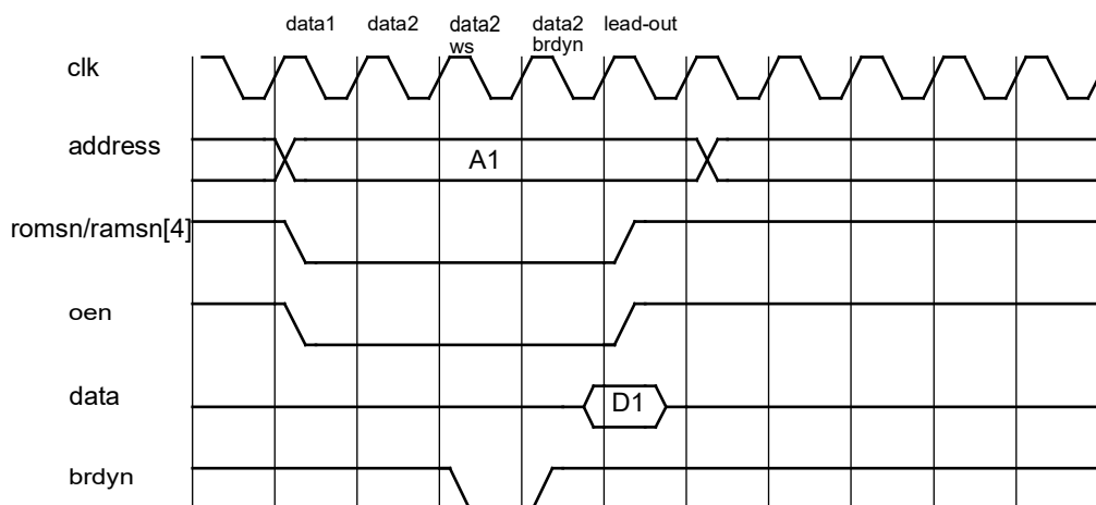
Figure 32. Read cycle with one waitstate (configured) and one BRDYN generated waitstate (synchronous sampling).
