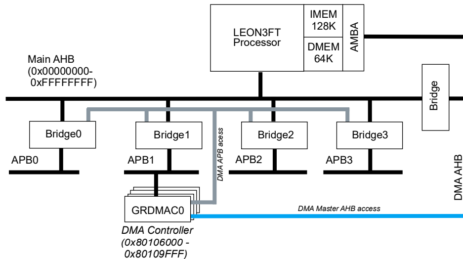
Figure 43. GR716A GRDMACx bus connection
