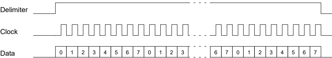
Figure 49. Synchronous bit serial waveform
