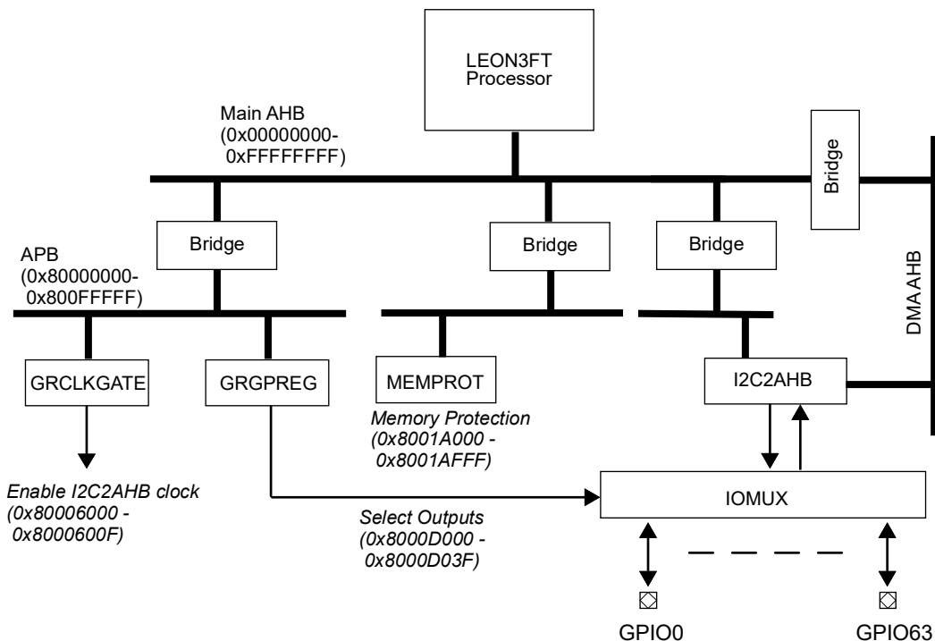
Figure 61. GR716A I2C2AHB bus and pin
