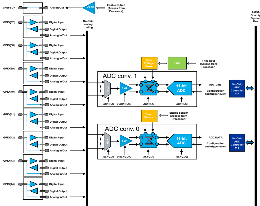
Figure 5. Shared external connections for ADC converter 0 and ADC converter 1.
