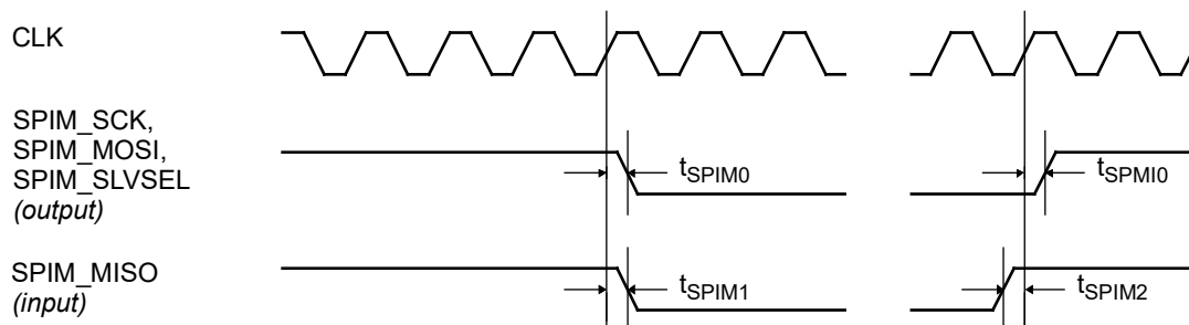
Figure 108. SPI interface timing waveforms
