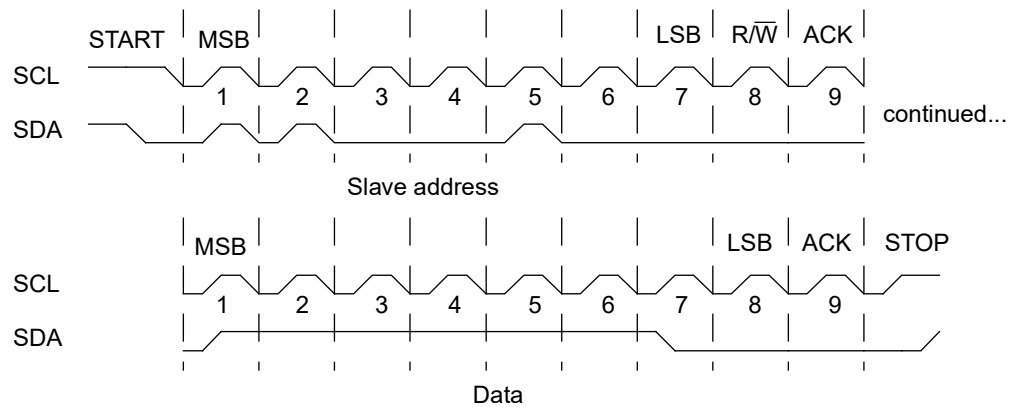
Figure 69. Complete I 2 C data transfer
