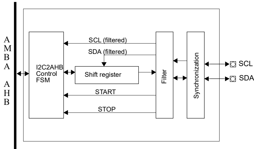
Figure 62. Block diagram
