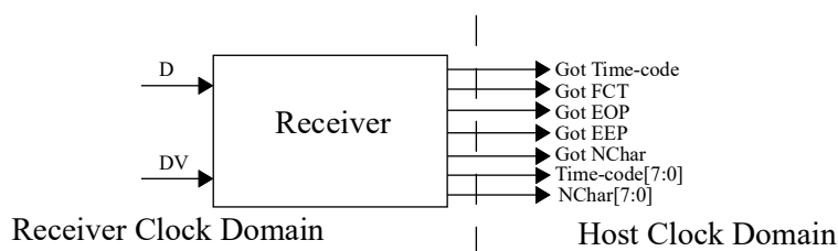
Figure 56. Schematic of the link interface receiver.
