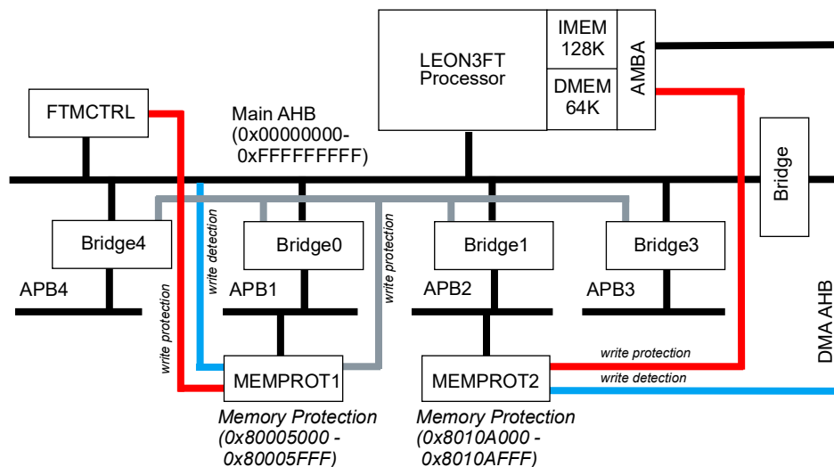
Figure 88. GR716A MEMPROTx bus connection
