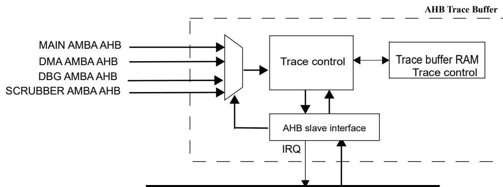
Figure 95. Block diagram
