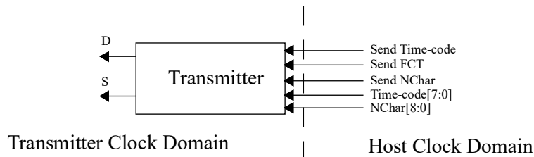
Figure 55. Schematic of the link interface transmitter.
