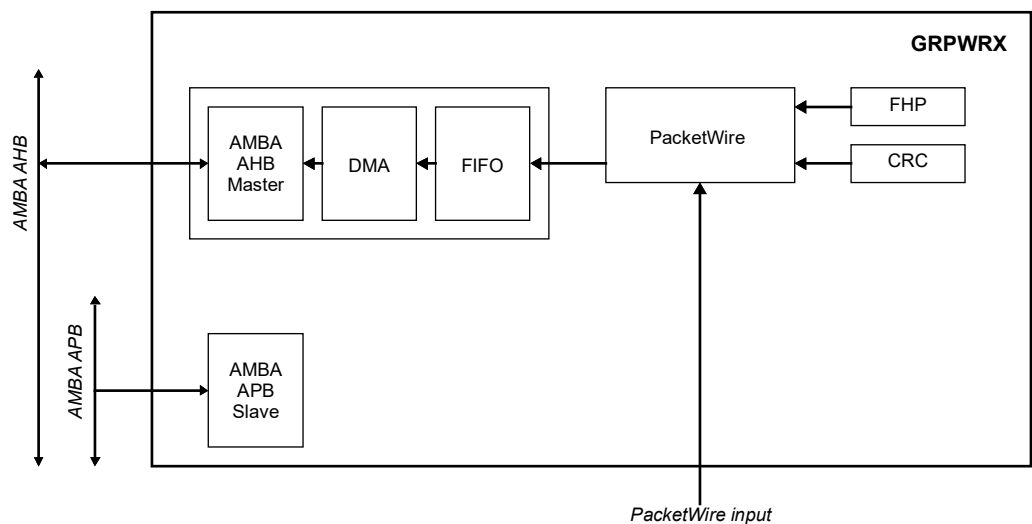
Figure 48. Block diagram
